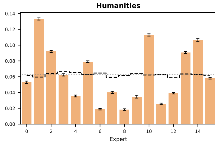
b4 — mean routing weight per expert by category (dashed = residual after subtracting global mean)
