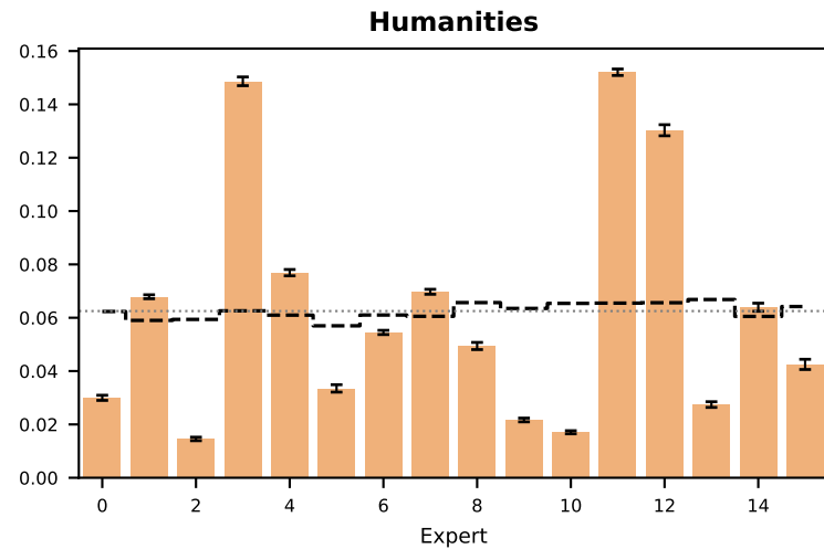
b5 — mean routing weight per expert by category (dashed = residual after subtracting global mean)
