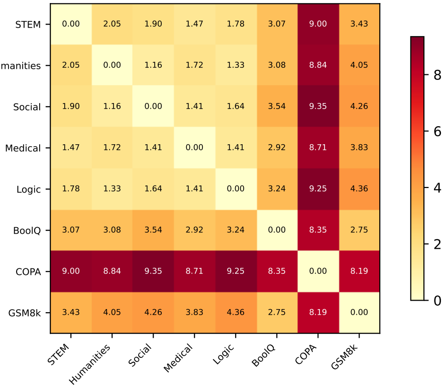
Mahalanobis distance (pooled cov)
