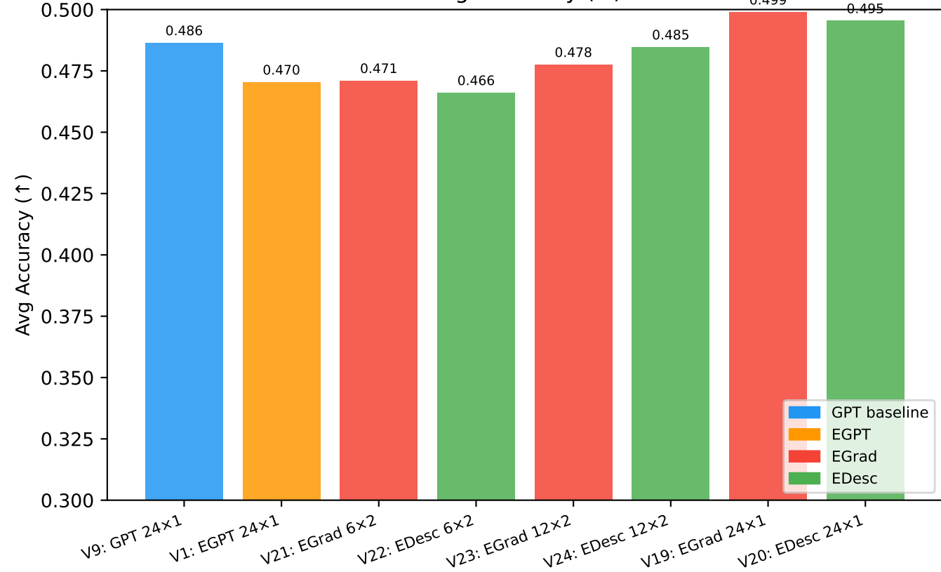
Avg Accuracy (↑)
