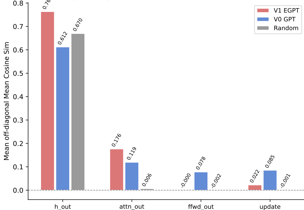
Inter-layer similarity (Mean Cosine Sim) (higher = layers produce more similar representations)
