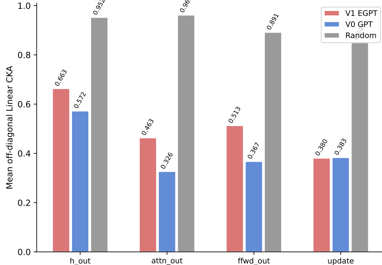
Inter-layer similarity (Linear CKA) (higher = layers produce more similar representations)
