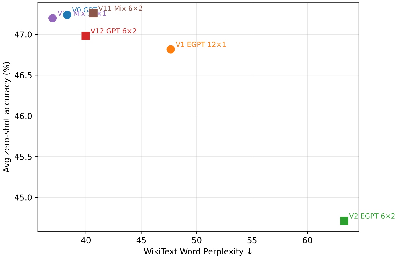
Accuracy vs Perplexity: iso-family (circles=12×1, squares=6×2)
