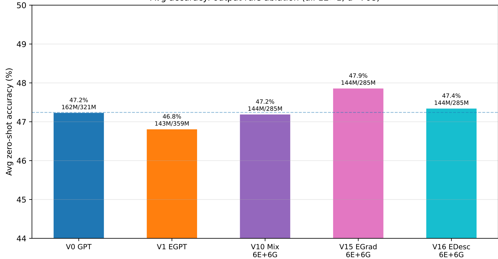
Avg accuracy: output rule ablation (all 12×1, d=768)
