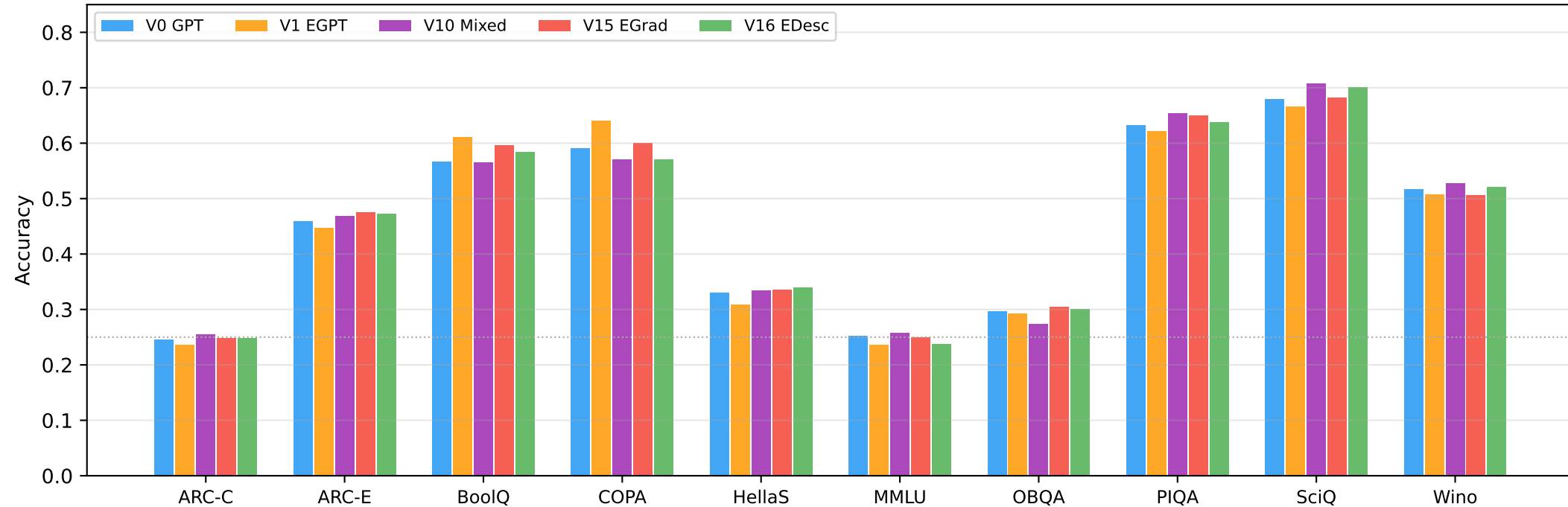
Output-rule ablation: V0 / V1 / V10 Mixed / V15 EGrad / V16 EDesc — per task
