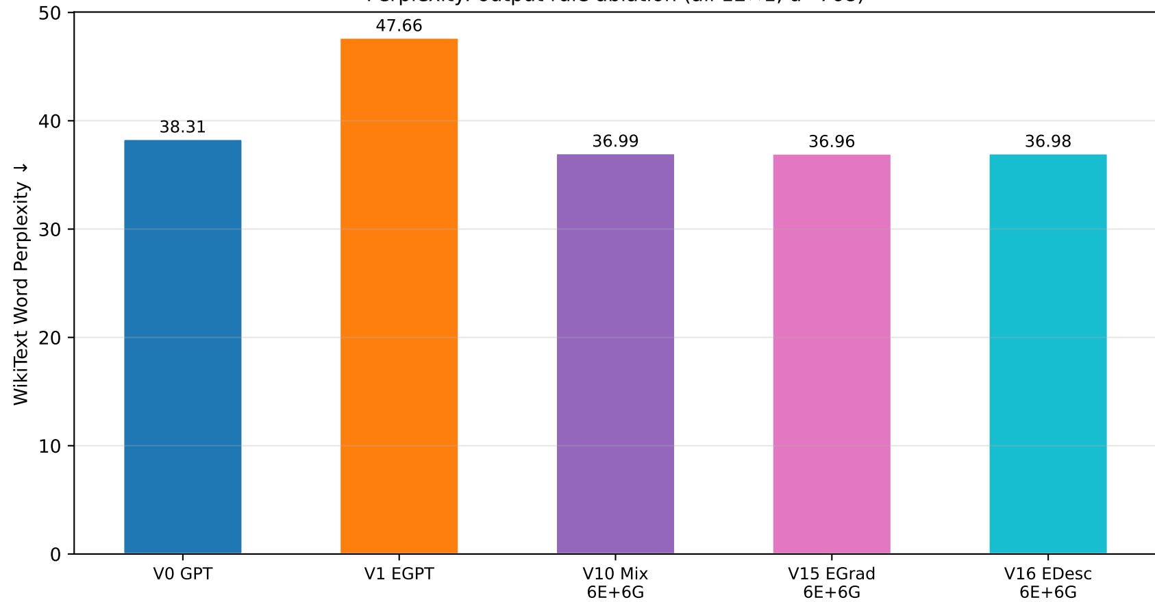
Perplexity: output rule ablation (all 12×1, d=768)
