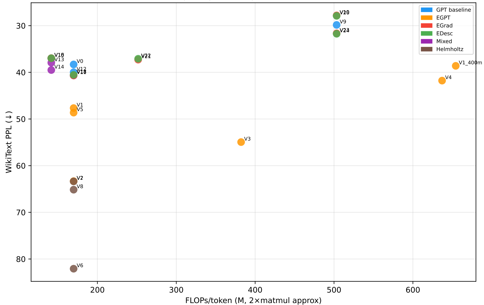
Perplexity vs Compute (FLOPs/token)
