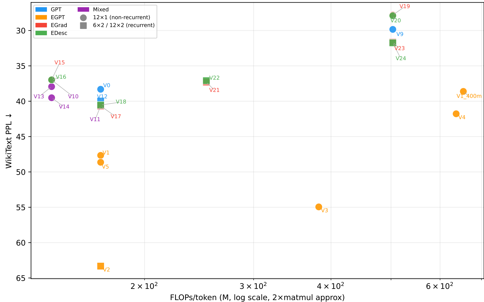
Perplexity vs Compute (no Helmholtz)
