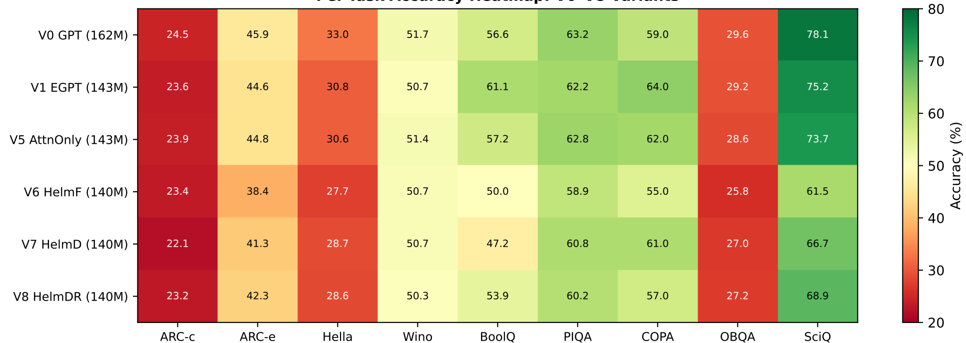
Per-Task Accuracy Heatmap: V0-V8 Variants
