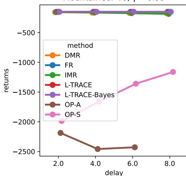
MountainCar-v0, \gamma = 0.99
