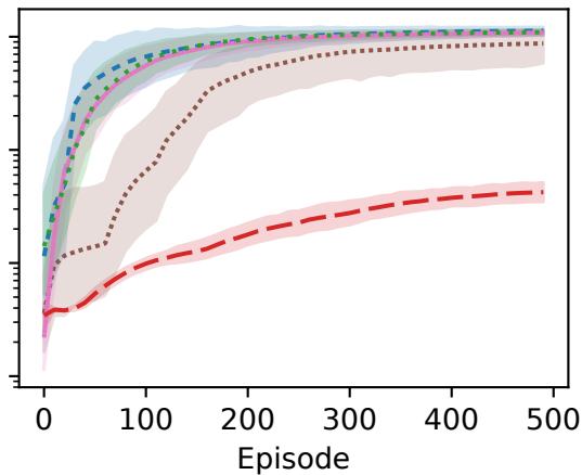
TC-PermExDc, \lambda = 4.0 Enc = tiles
