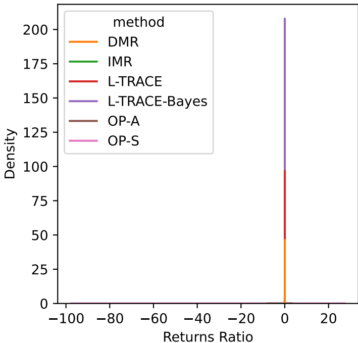
Environment = RedGreen-v0
