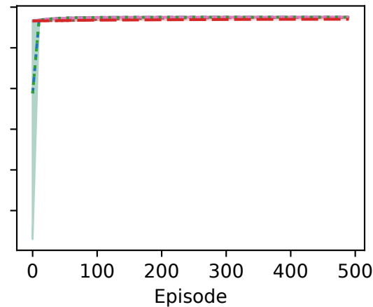
TC-PermExDc, \lambda = 4.0 Enc = tiles
