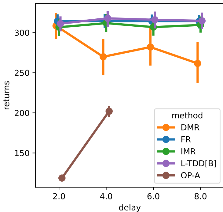
Finite-SC-PermExDc-v0, \gamma = 1.0
