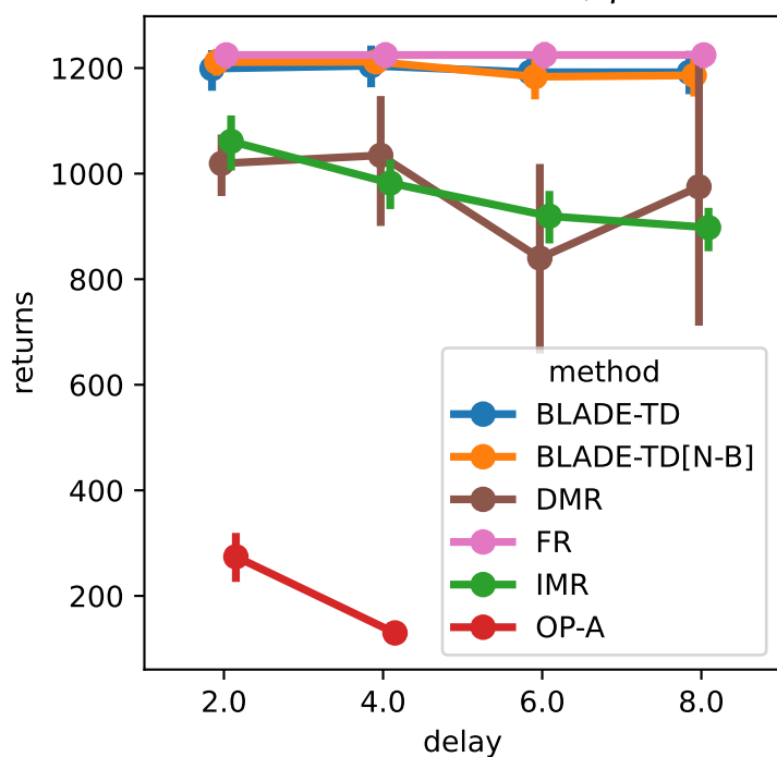
Finite-TC-PermExDc-v0, \gamma = 0.99
