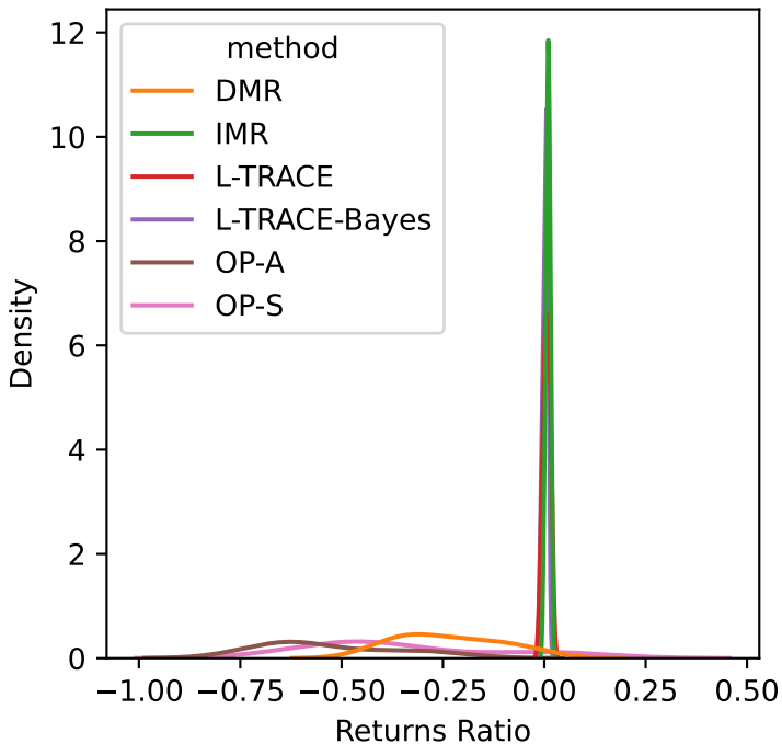
Environment = Finite-SC-PermExDc-v0
