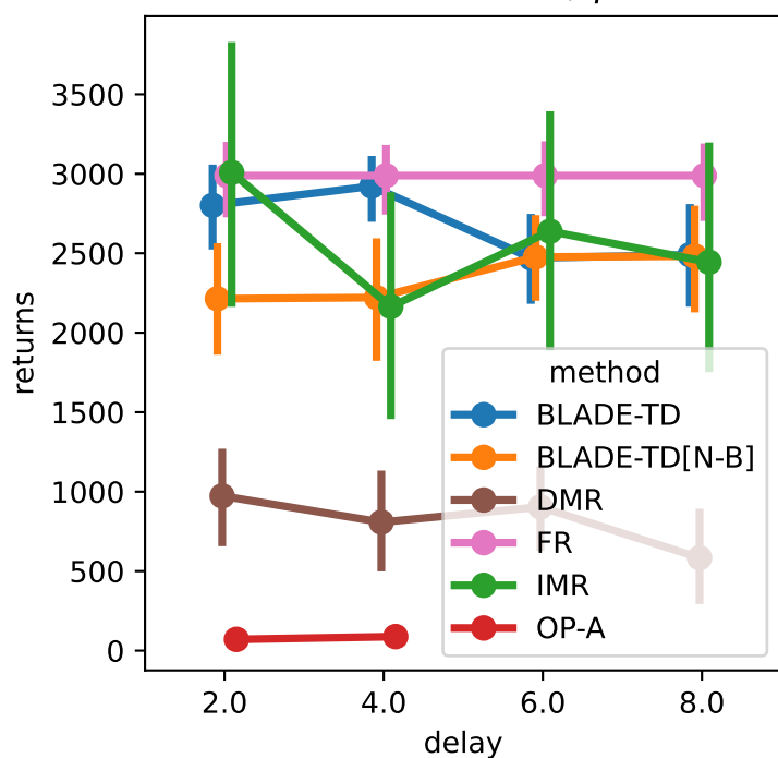
Finite-TC-ShuntDc-v0, \gamma = 0.99
