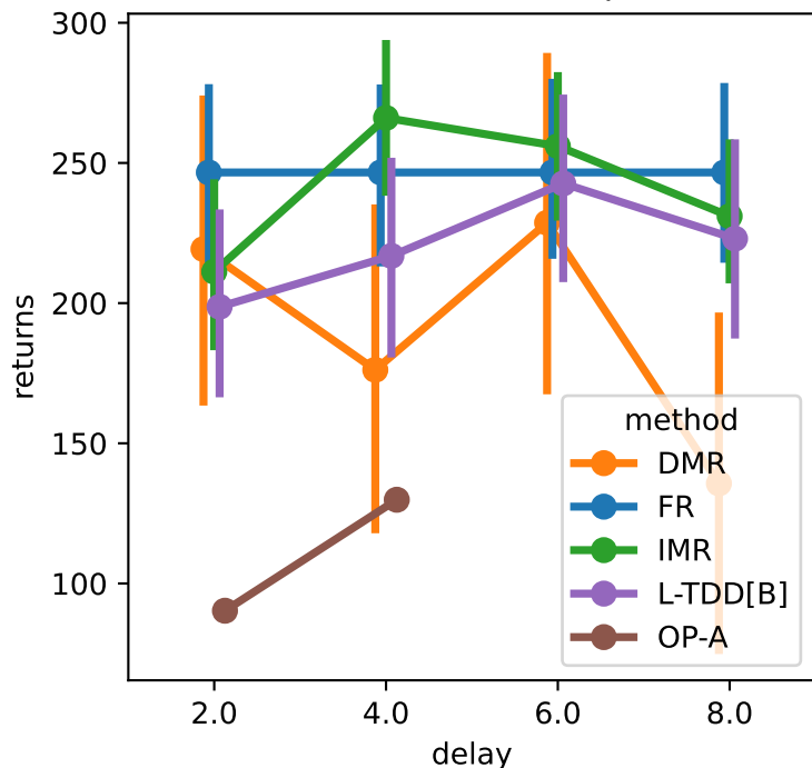
Finite-TC-ShuntDc-v0, \gamma = 0.99
