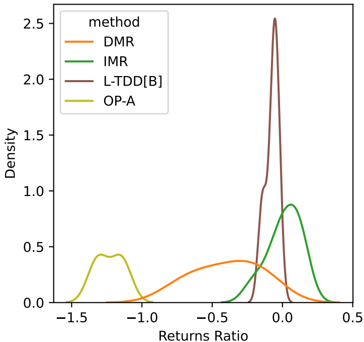
Environment = IceWorld-v0
