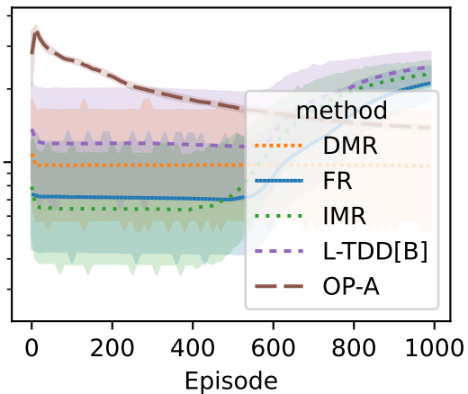
TC-ShuntDc-v0, \lambda = 4.0 Enc = scale
