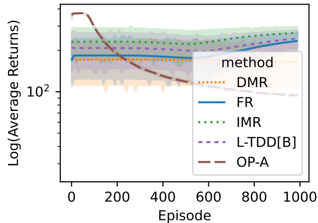
TC-ShuntDc-v0, \lambda = 2.0 Enc = scale
