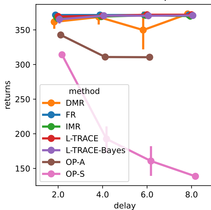
Finite-TC-PermExDc-v0, \gamma = 1.0
