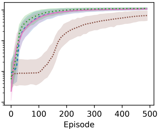
TC-PermExDc, \lambda = 6.0 Enc = tiles
