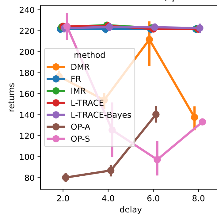
GridWorld-v0, \gamma = 0.99
