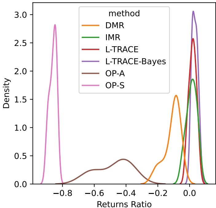
Environment = Finite-CC-PermExDc-v0
