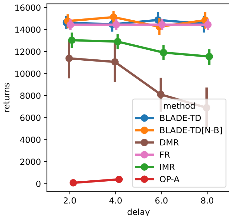
Finite-TC-PermExDc-v0, \gamma = 0.99
