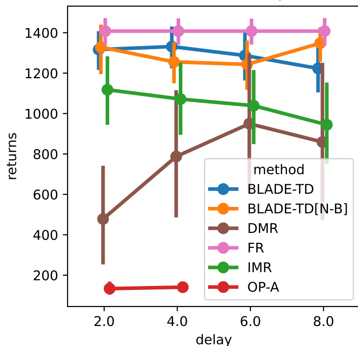
Finite-TC-ShuntDc-v0, \gamma = 1.0
