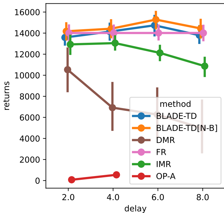
Finite-SC-PermExDc-v0, \gamma = 0.99
