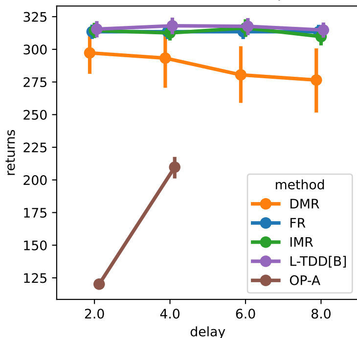
Finite-TC-PermExDc-v0, \gamma = 1.0
