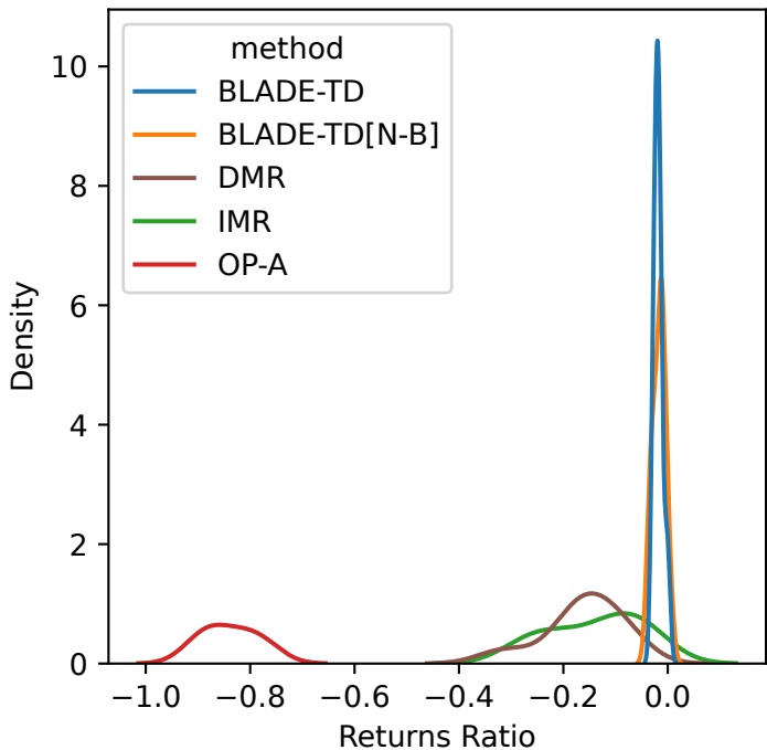
Environment = Finite-SC-PermExDc-v0
