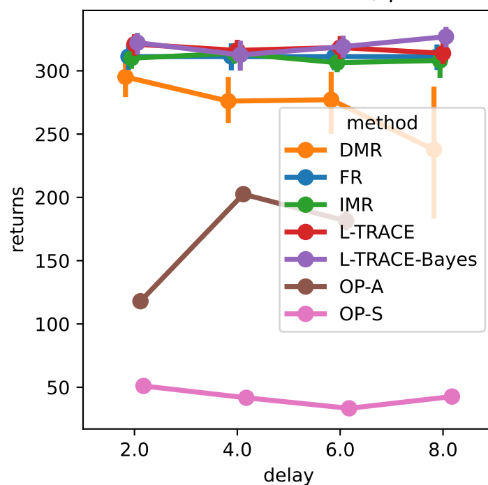
MountainCar-v0, \gamma = 1.0
