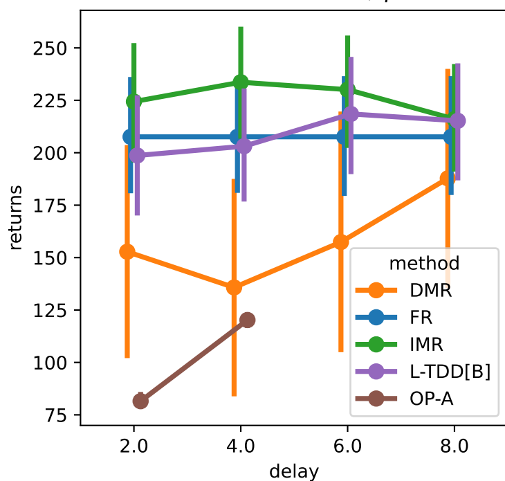
Finite-TC-ShuntDc-v0, \gamma = 1.0
