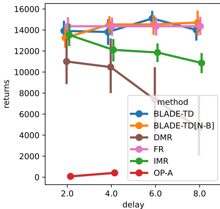
Finite-SC-PermExDc-v0, \gamma = 0.99
