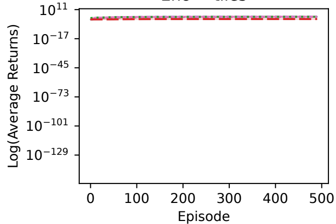
TC-PermExDc, \lambda = 2.0 Enc = tiles
