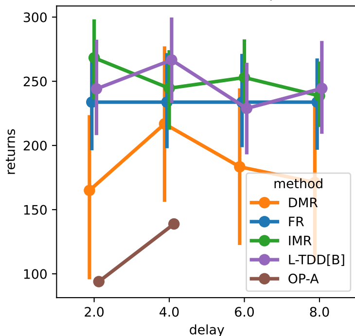
Finite-TC-ShuntDc-v0, \gamma = 1.0
