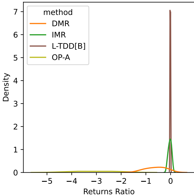
Environment = GridWorld-v0
