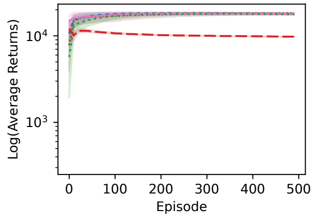
CC-ShuntDc, \lambda = 2.0 Enc = tiles
