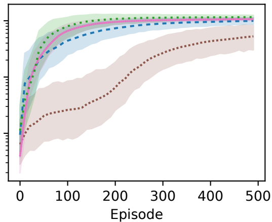
CC-PermExDc, \lambda = 6.0 Enc = spliced-tiles
