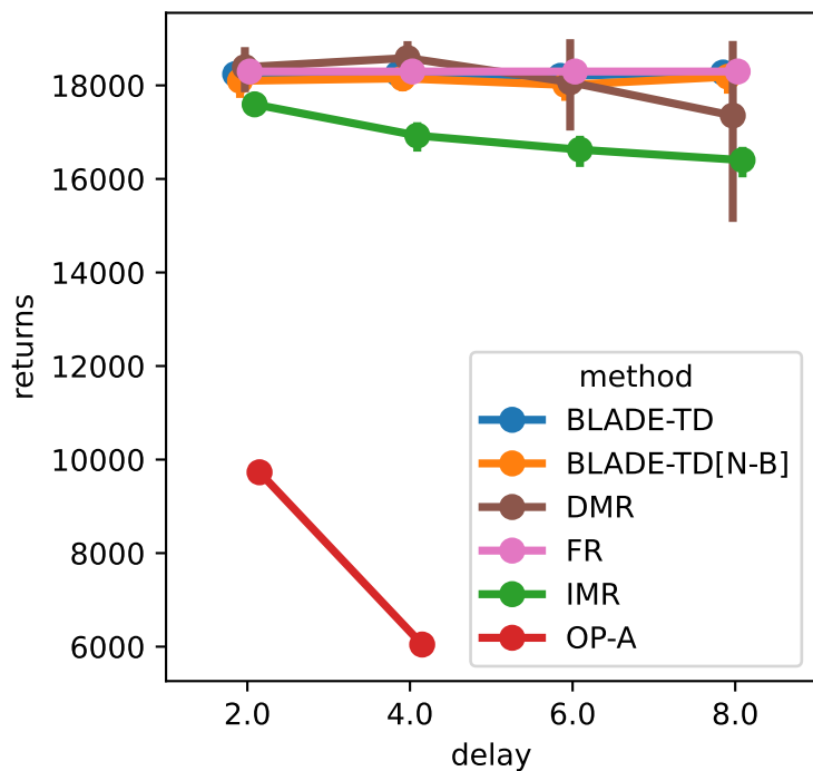
Finite-SC-ShuntDc-v0, \gamma = 0.99
