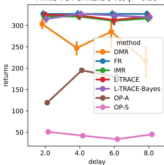
MountainCar-v0, \gamma = 0.99
