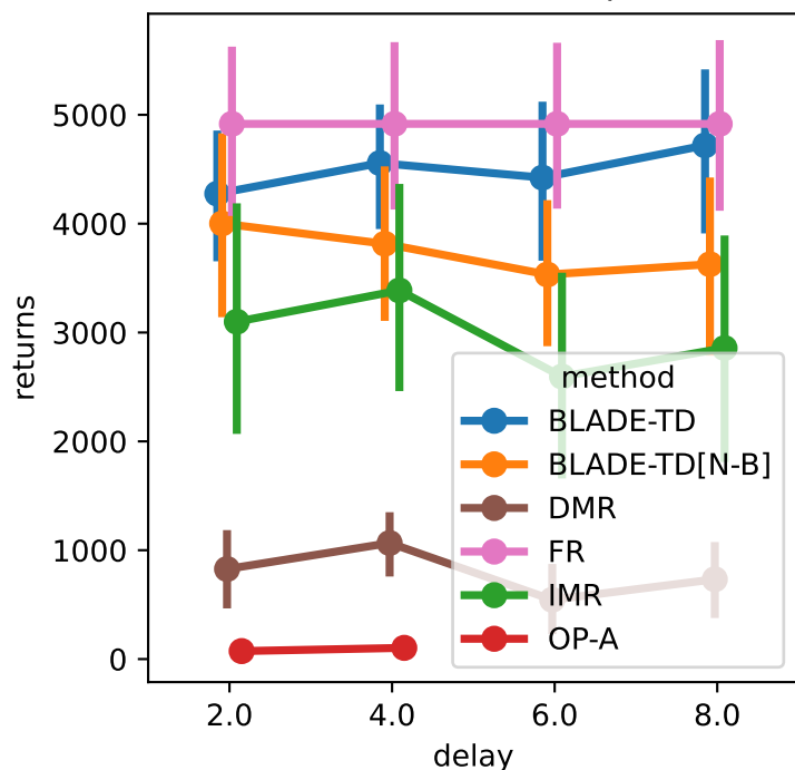
Finite-TC-ShuntDc-v0, \gamma = 0.99
