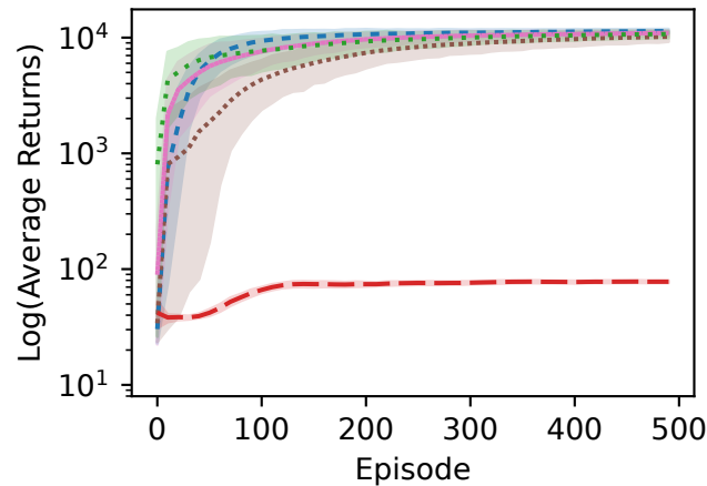
TC-PermExDc, \lambda = 2.0 Enc = tiles
