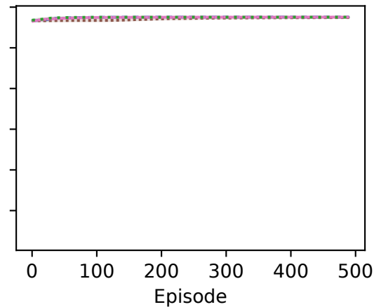
TC-PermExDc, \lambda = 6.0 Enc = tiles
