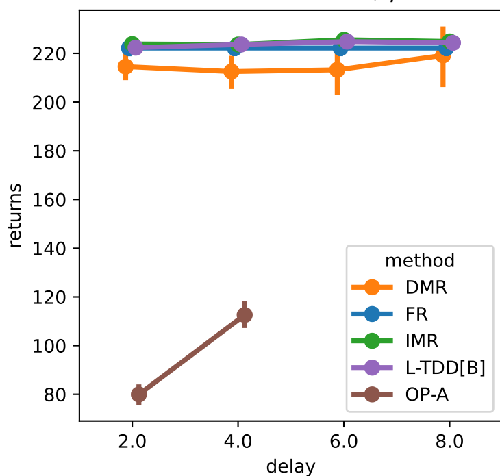
Finite-TC-PermExDc-v0, \gamma = 1.0
