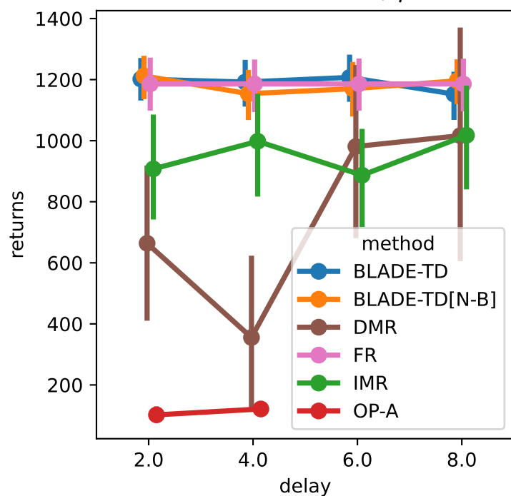
Finite-TC-ShuntDc-v0, \gamma = 1.0
