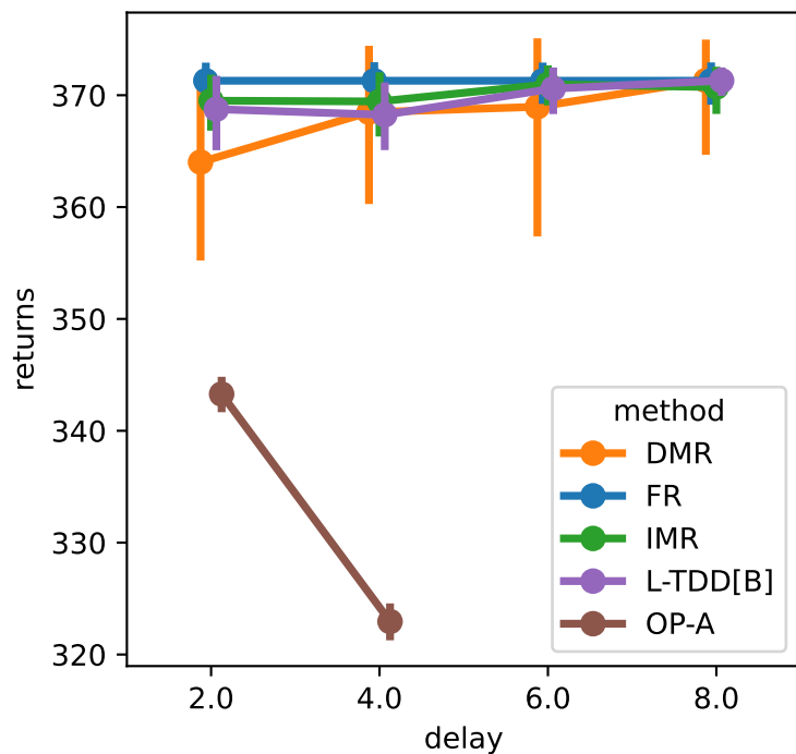
Finite-SC-ShuntDc-v0, \gamma = 1.0
