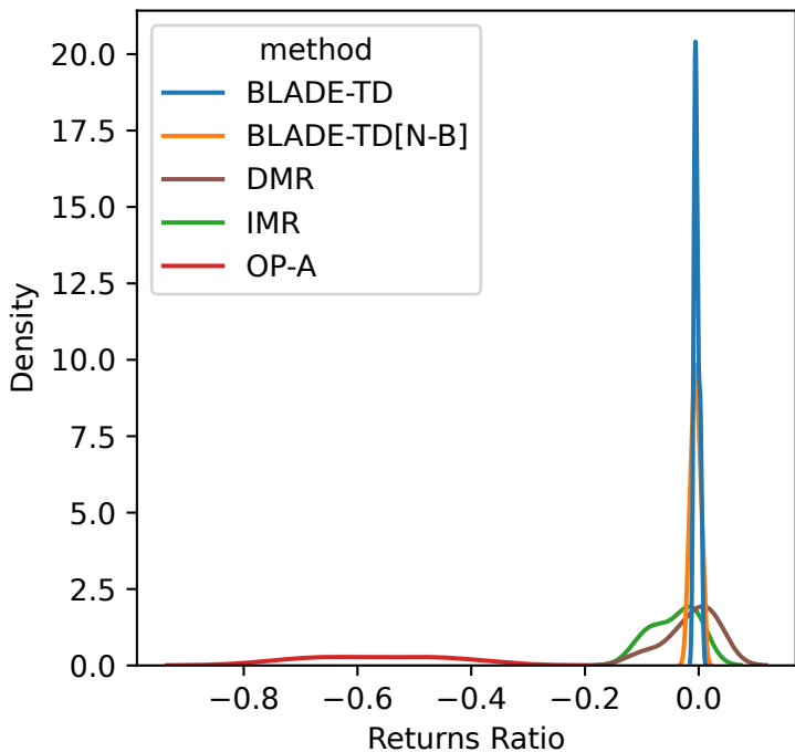
Environment = Finite-CC-ShuntDc-v0
