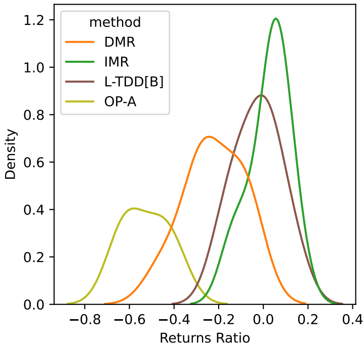
Environment = Finite-TC-ShuntDc-v0
