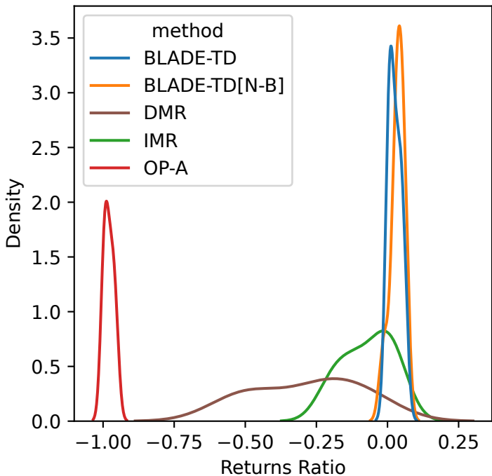
Environment = Finite-TC-PermExDc-v0
