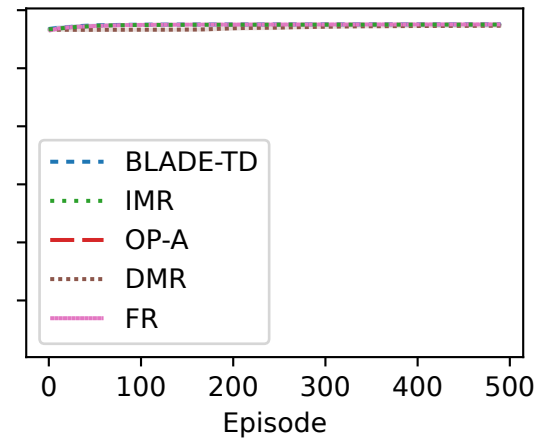
TC-PermExDc, \lambda = 8.0 Enc = tiles
