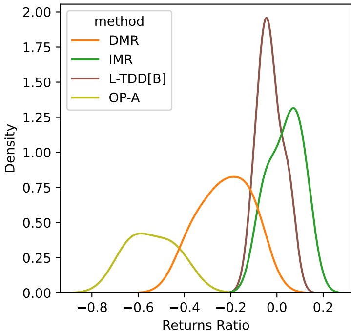
Environment = Finite-SC-ShuntDc-v0
