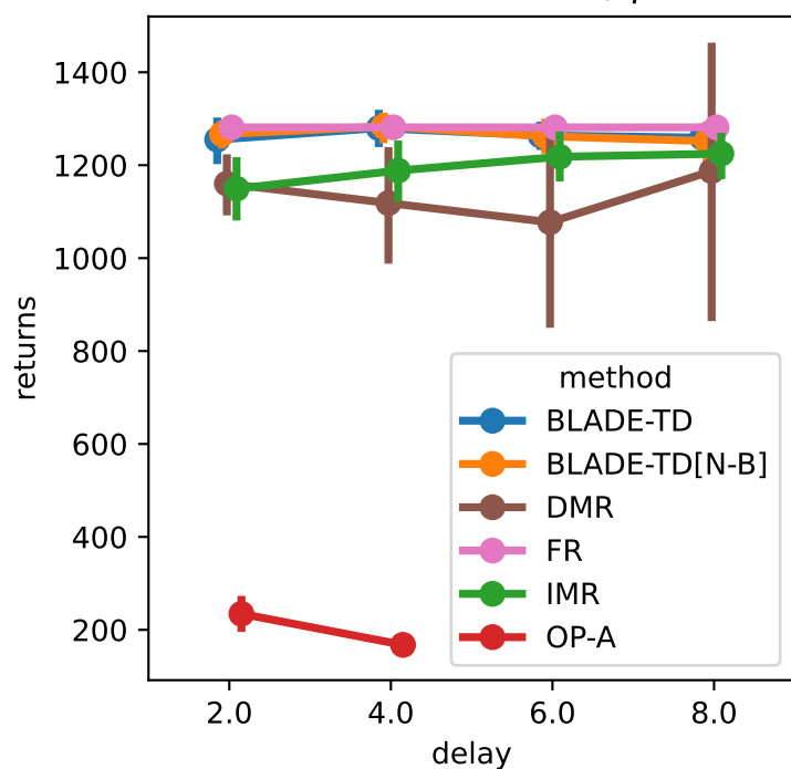
Finite-TC-PermExDc-v0, \gamma = 1.0
