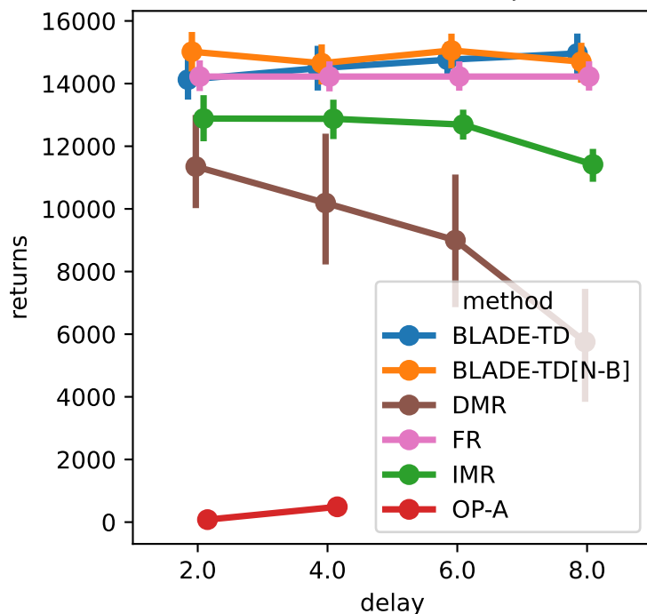
Finite-TC-PermExDc-v0, \gamma = 0.99
