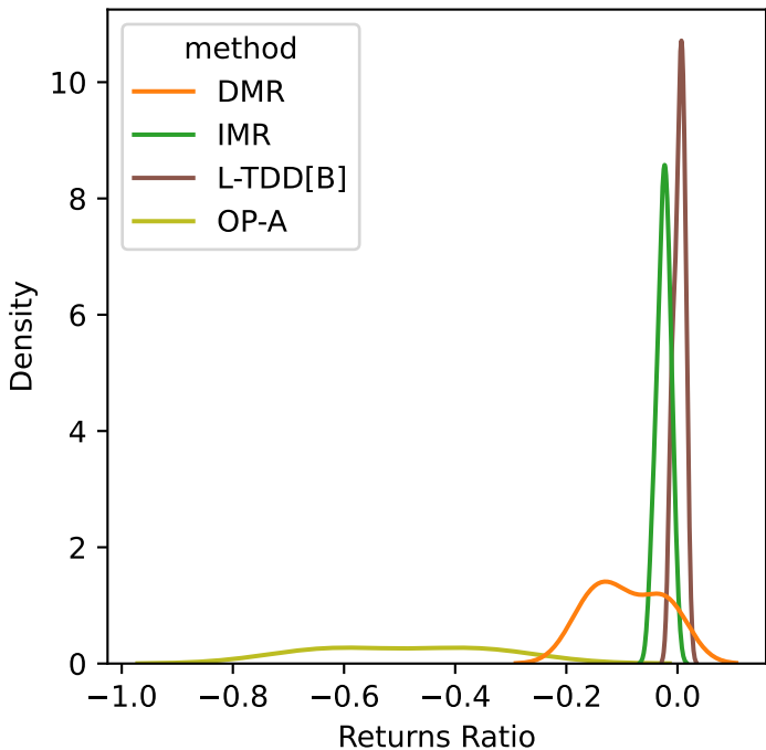
Environment = Finite-CC-PermExDc-v0
