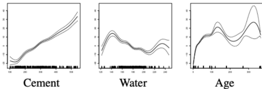
Figure 2: Cement : monotonically increasing — more cement, higher strength. Water : non-monotone — there is an optimal range; too much or too little reduces strength. Age : rapid early growth (curing process), stabilizes with a second soft peak at later ages.
