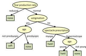
Decision trees
