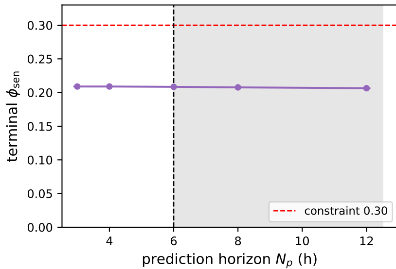
Prediction-horizon sweep at N_c = 3 (shaded region: N_p beyond the 6 h window)
