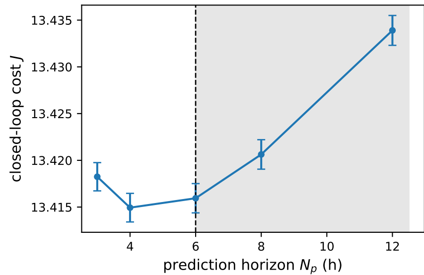
Prediction-horizon sweep at N_c = 3 (shaded region: N_p beyond the 6 h window)
