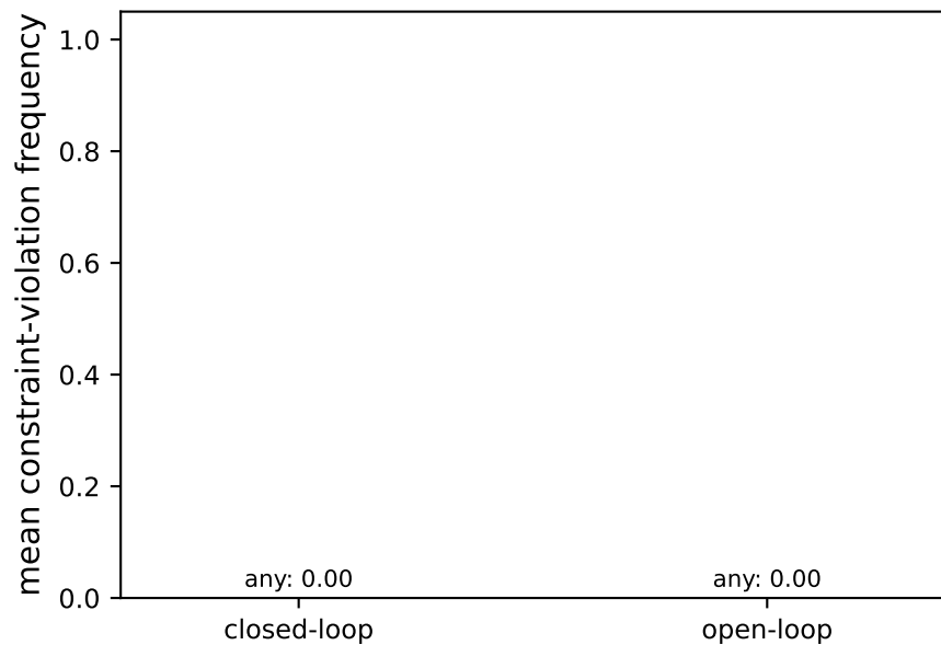
(b) constraint violation, feedback vs feedforward
