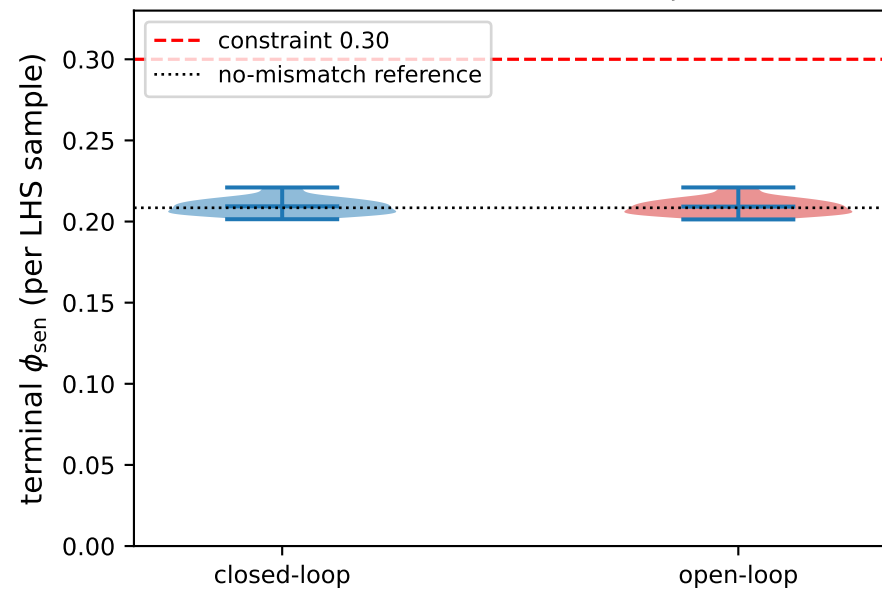
(a) terminal senescent fraction under joint mismatch
