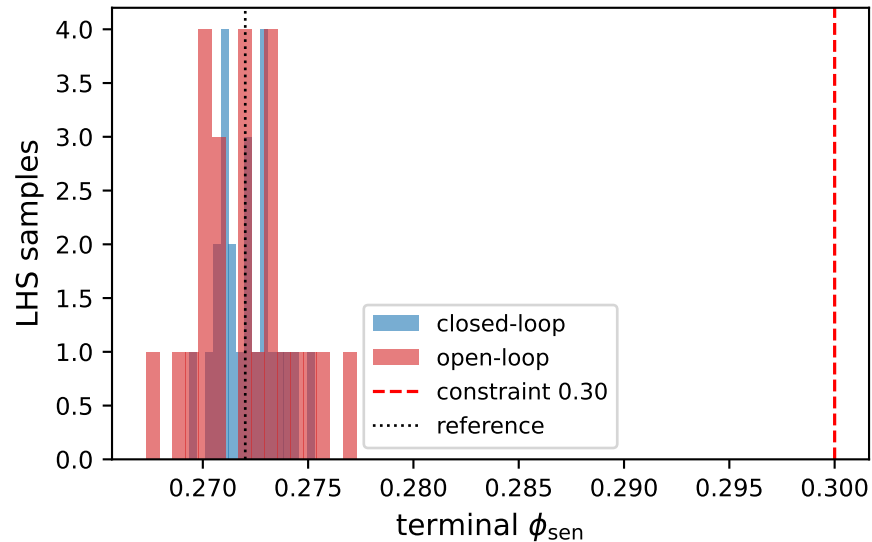
(a) terminal senescent fraction
