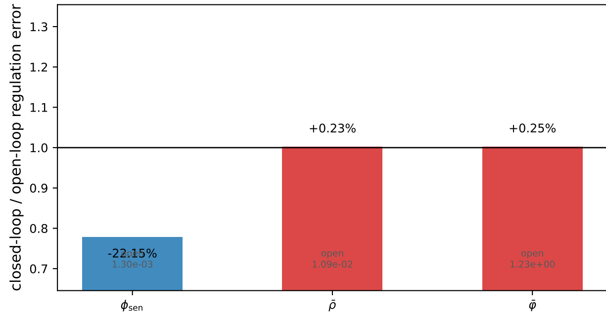
Feedback correction of the regulation error under joint mismatch (below one, feedback reduces the error; above one, feedforward is better)
