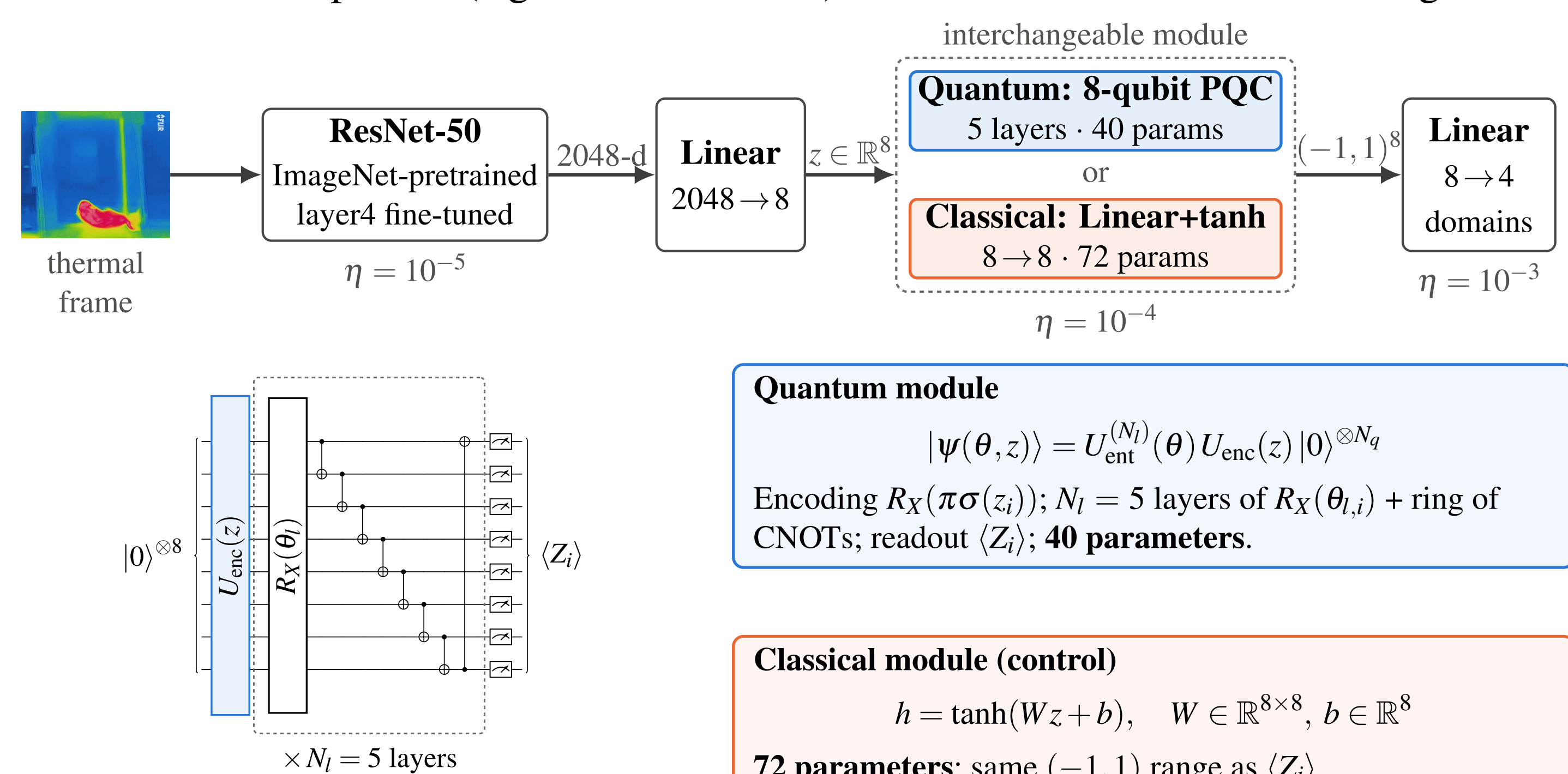
Figure 2: Paired ablation: shared pipeline (top); quantum circuit vs classical block (bottom).
