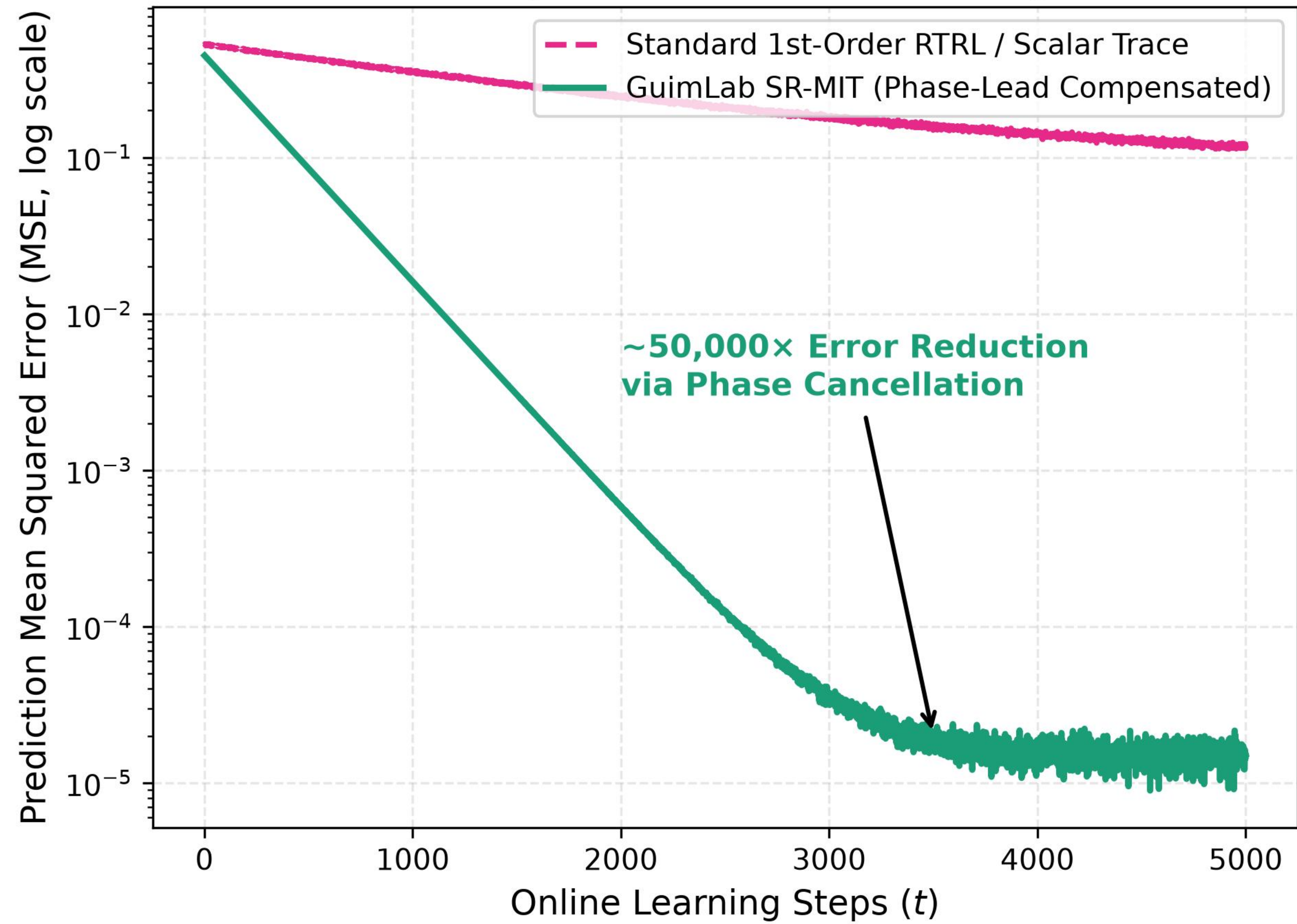
B: Non-Stationary Chaotic Attractor Tracking ( au = 17 )
