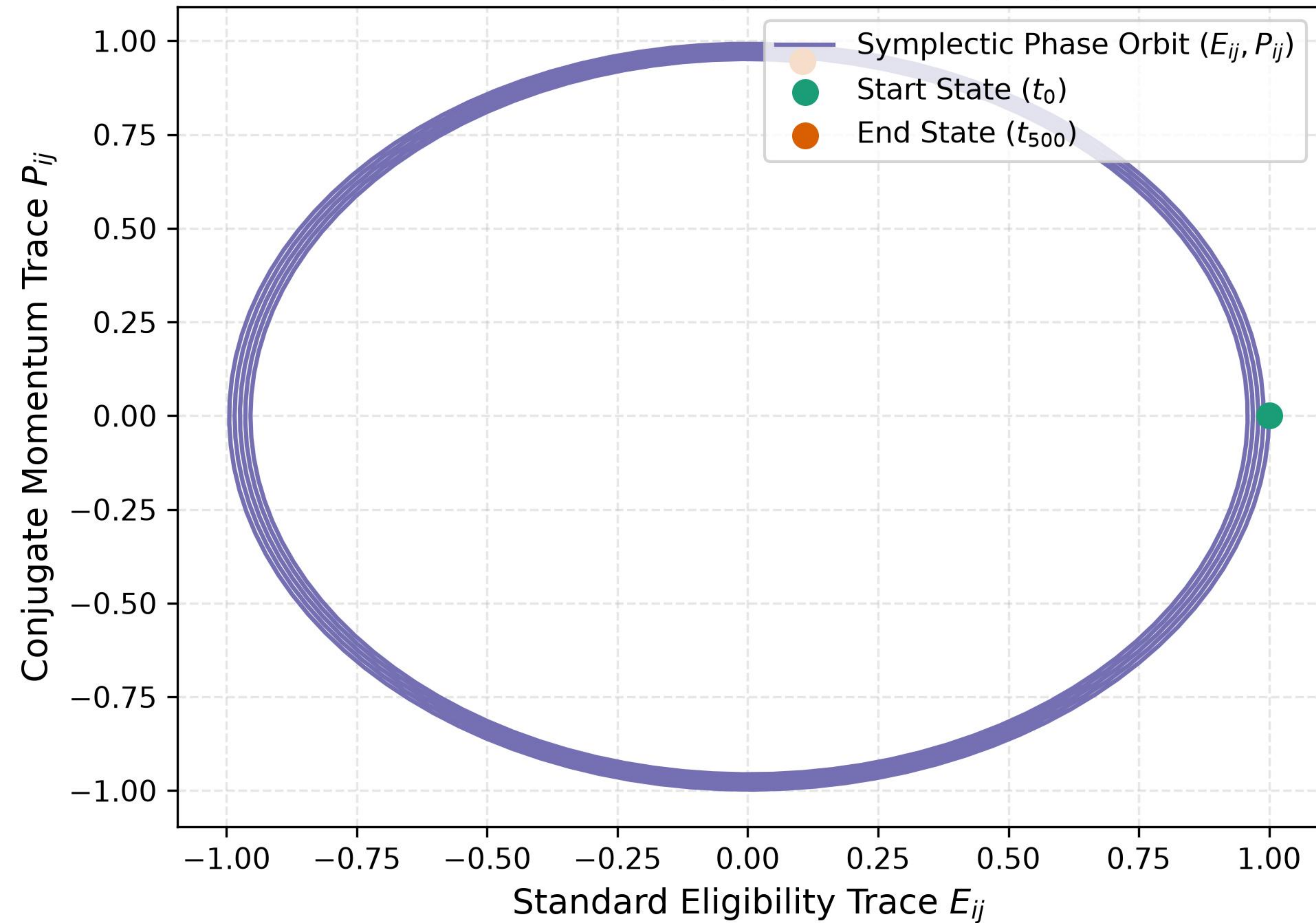
A: SR-MIT 2-Form Symplectic Phase Space
