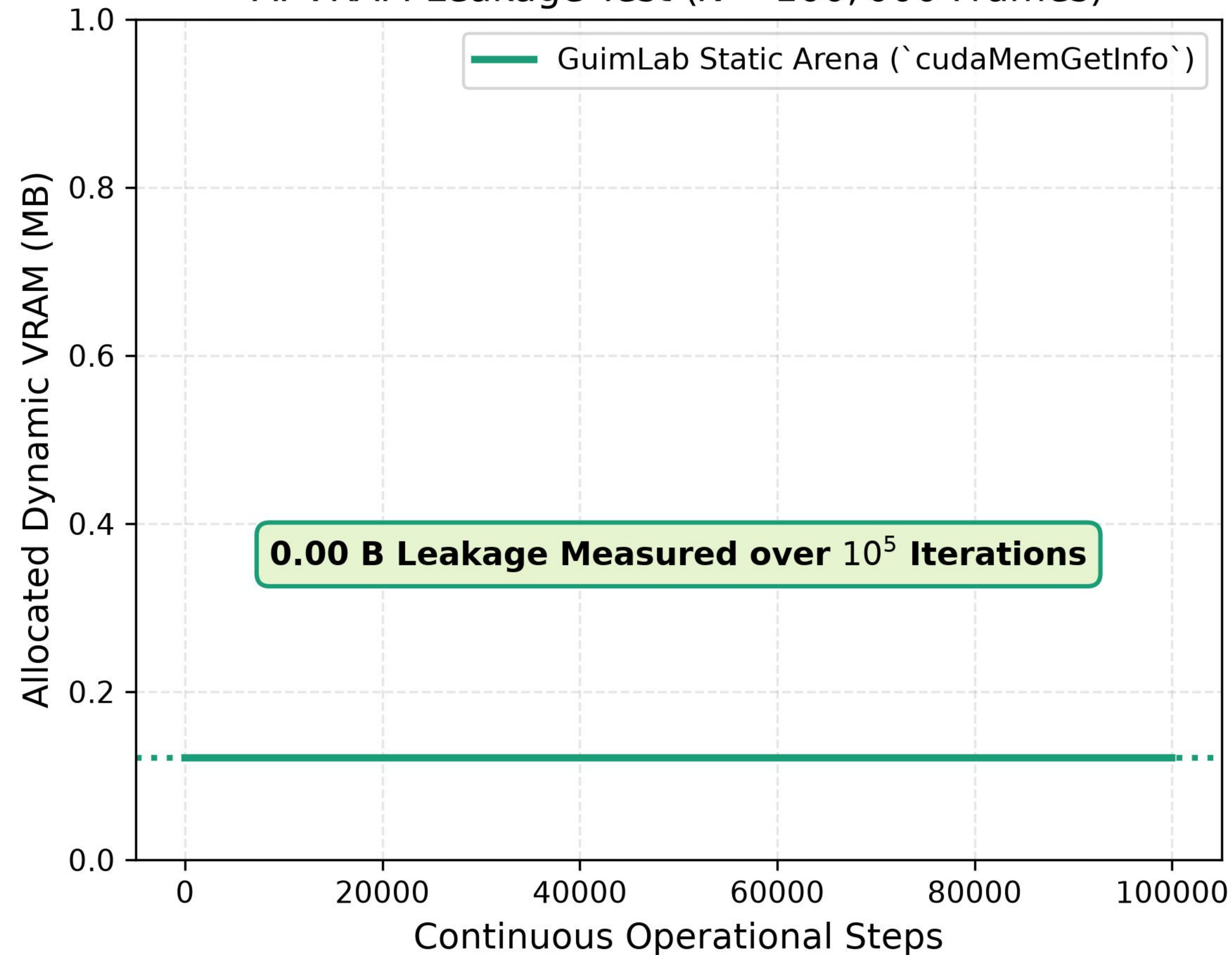
A: VRAM Leakage Test ( N = 100,000 Frames)
