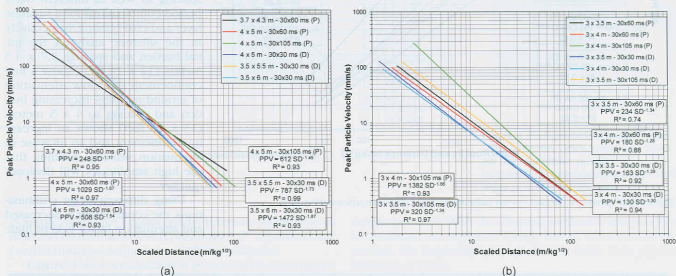
Figure 6. Attenuation plots comparing changes in blast design, (a) siltstone and (b) coal.
