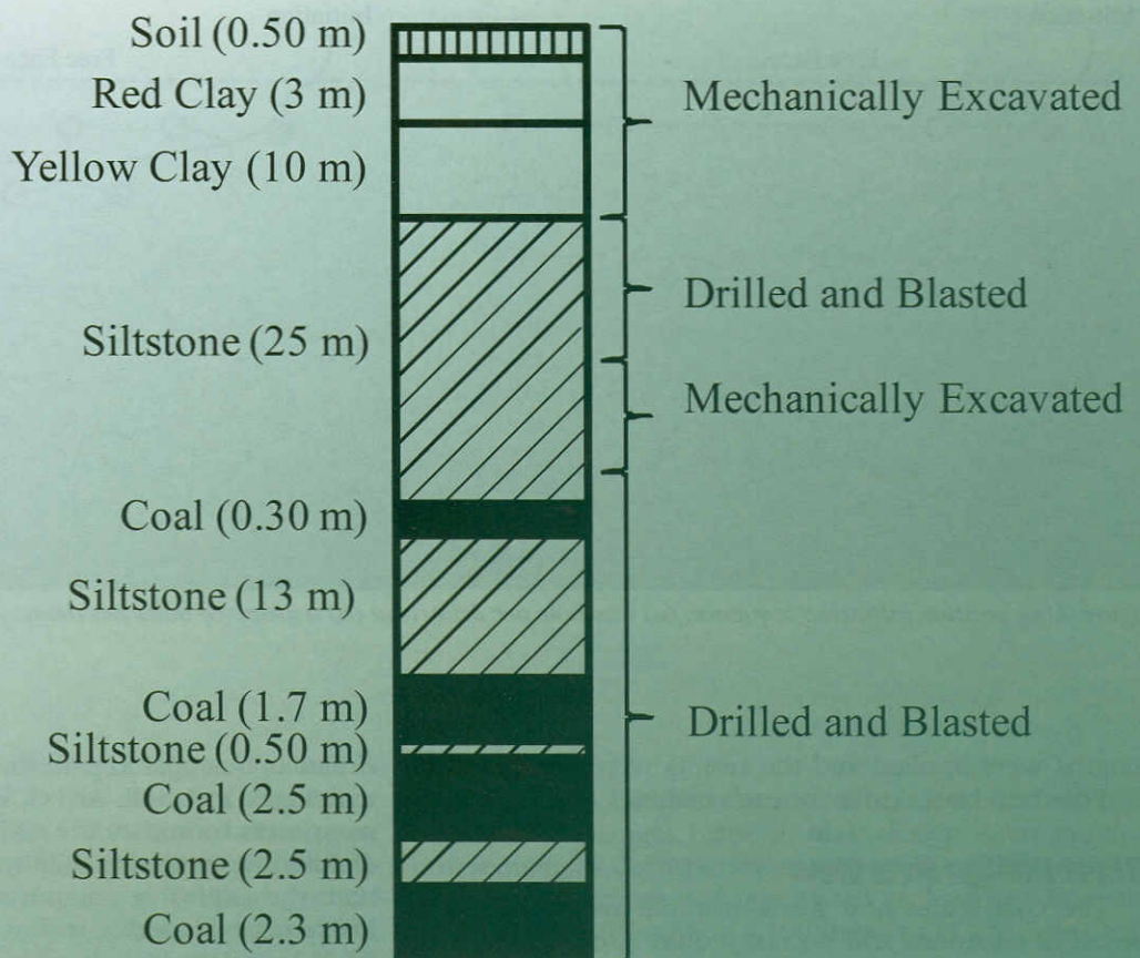
Figure 1. Coal deposit profile.
