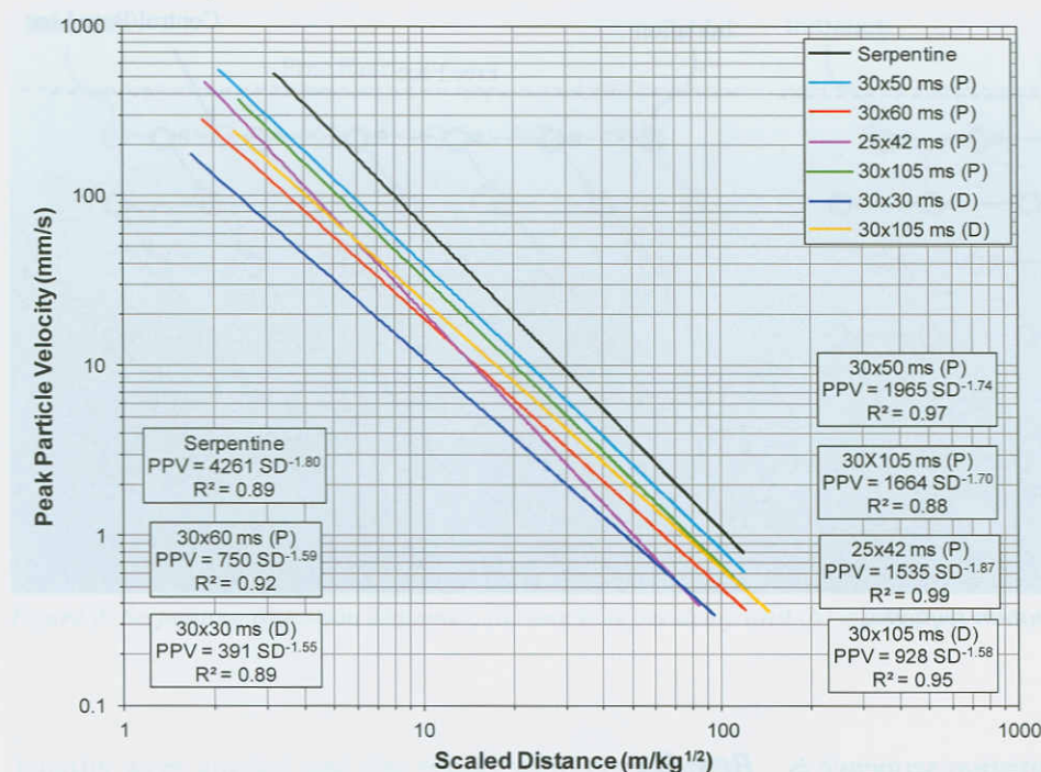
Figure 4. Peak particle velocity versus scaled distance attenuation plot comparing serpentine, parallel (P) and diagonal (D) initiation sequences and delay period combinations.
