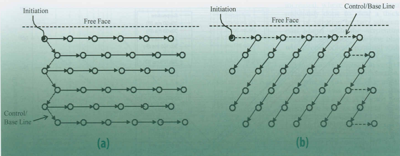
Figure 3. (a) Parallel and (b) diagonal initiation sequence.
