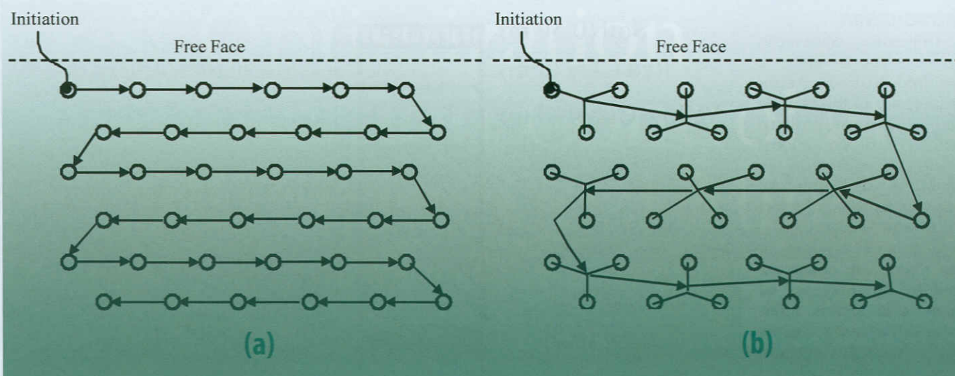
Figure 2. Serpentine initiation sequence, (a) one hole per delay and (b) a group of holes per delay.
