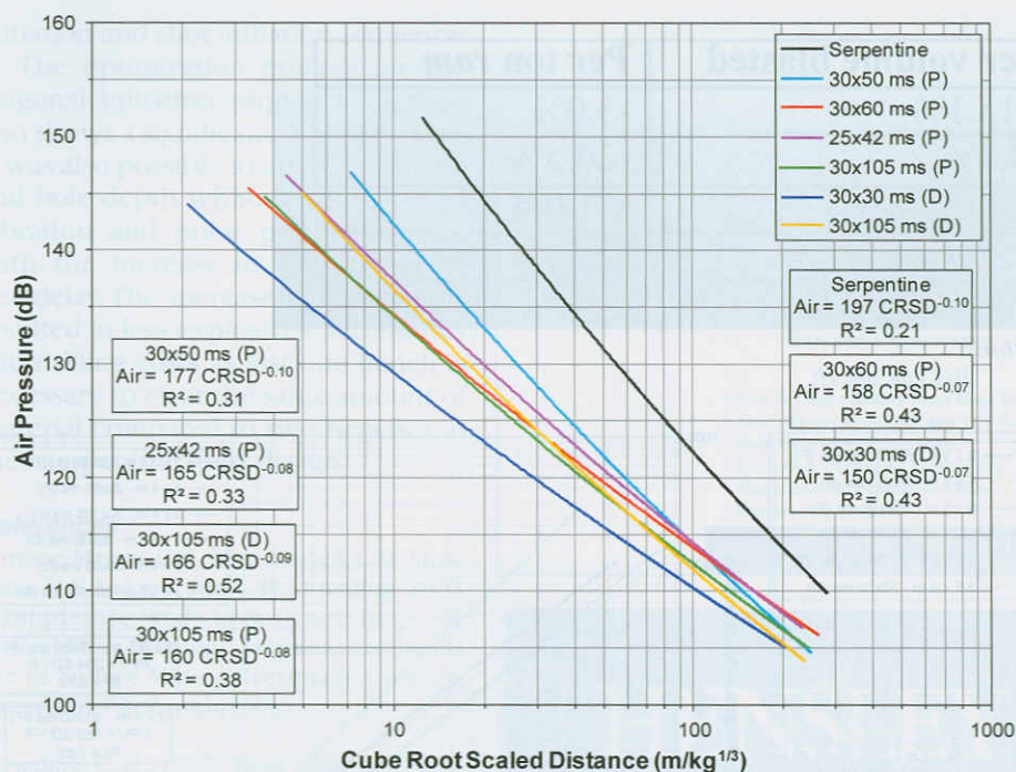
Figure 5. Air pressure (noise) versus cube root scaled distance attenuation plot.
