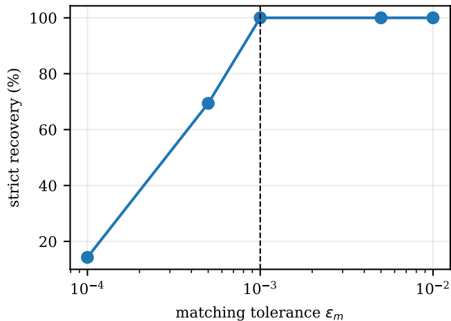
(c) Smooth quartic objectives (30 trials)
