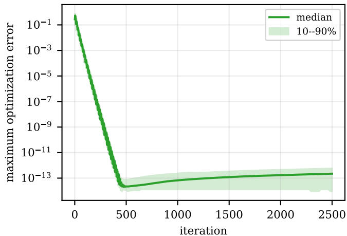
(c) Smooth quartic objectives (30 trials)
