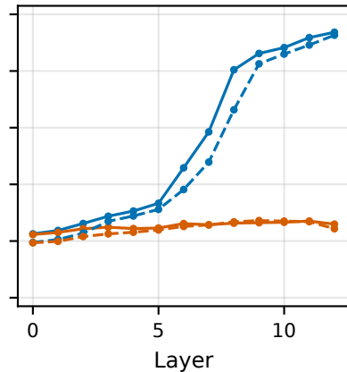
HEAD (positional)
