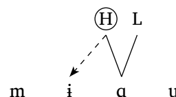
Figure 43: Contour tone
