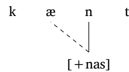
Figure 39: Feature spreading
