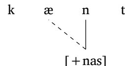
Figure 39: Feature spreading
