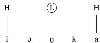
Figure 42: Floating tone
