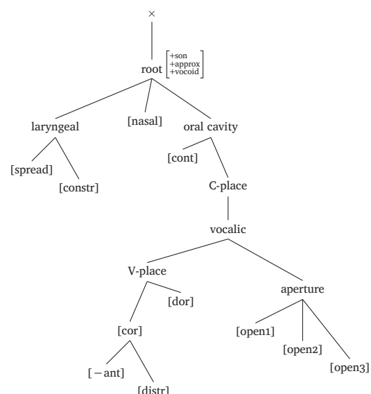
Figure 52: Vocoids
