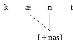
Figure 39: Feature spreading
