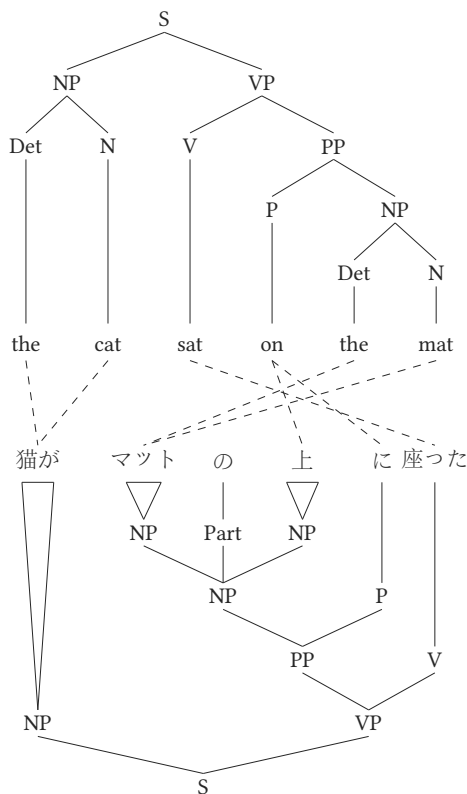
Tree 11: Bilingual trees — adapted from Chiang's tutorial on tikz-qtrees
