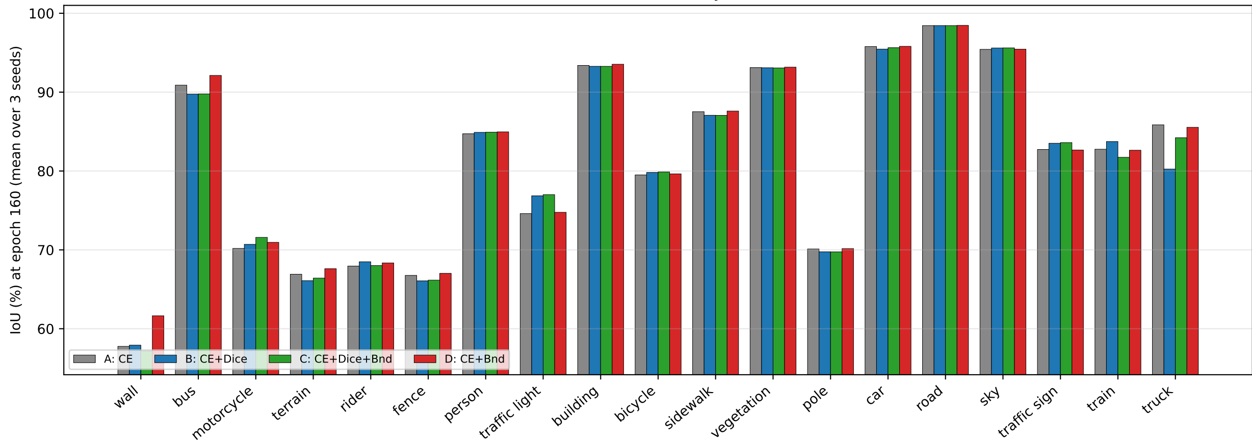
Per-class IoU — sorted by \Delta(D - A)
