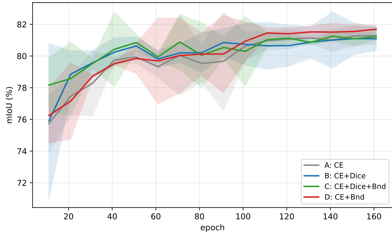
Per-epoch mIoU (mean over 3 seeds, 95% Student-t CI)
