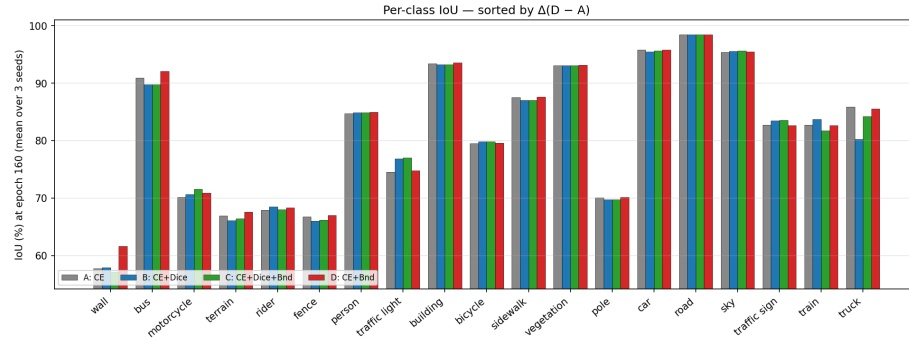
Figure 2: Per-class IoU
