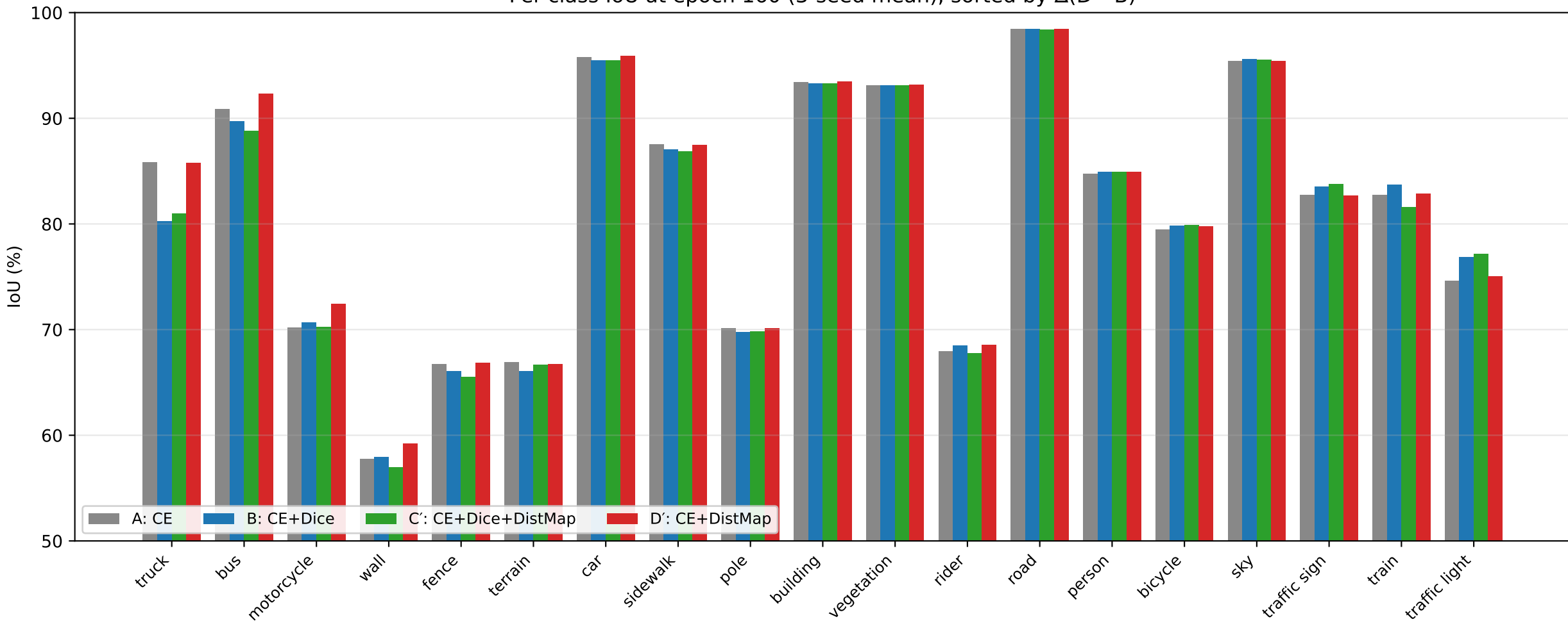
Per-class IoU at epoch 160 (3-seed mean), sorted by \Delta(D'-B)
