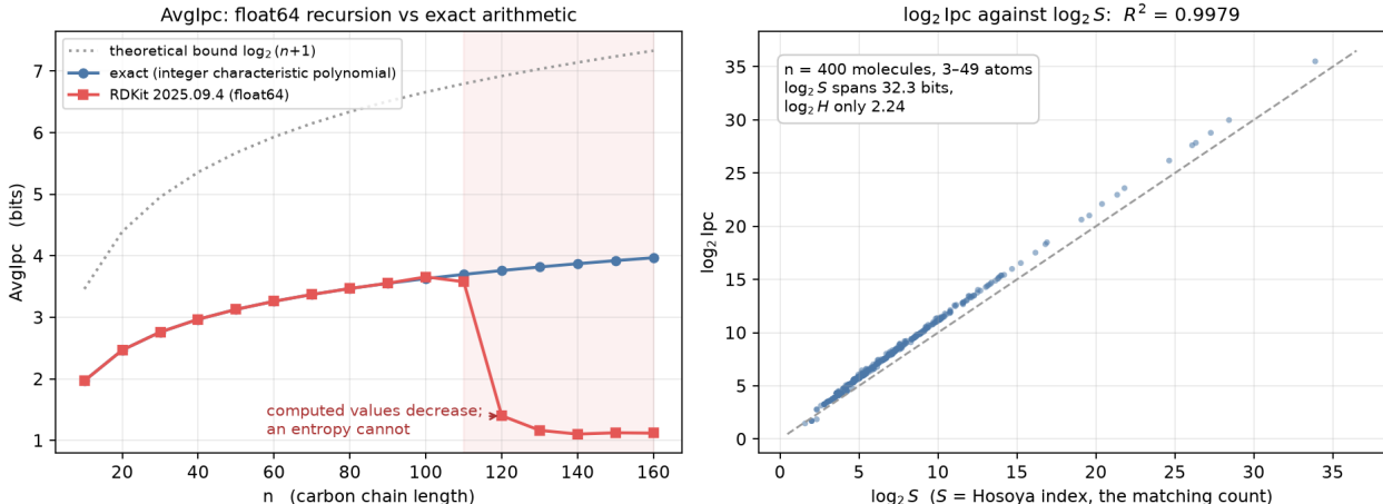
Figure 1: Left: AvgIpc from RDKit 2025.09.4 compared with exact integer arithmetic for linear carbon chains, n = 10 –160; dotted line is the bound \log_2(n+1) . Right: \log_2 \text{Ipc} against \log_2 S for 400 molecules of 3–49 heavy atoms; dashed line is y = x .
