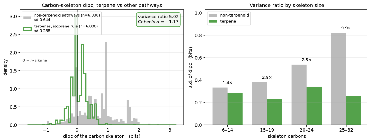
Figure 3: Left: dLPC of the carbon skeleton for 6,000 structurally defined terpenes and 6,000 non-terpenoid natural products matched on skeleton carbon count. Right: standard deviation by skeleton size, variance ratio annotated.
