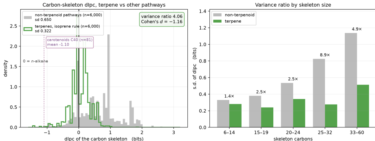
Figure 3: Left: dIpc of the carbon skeleton for 6,000 structurally defined terpenes and 6,000 non-terpenoid natural products matched on skeleton carbon count. Right: standard deviation by skeleton size, variance ratio annotated.
