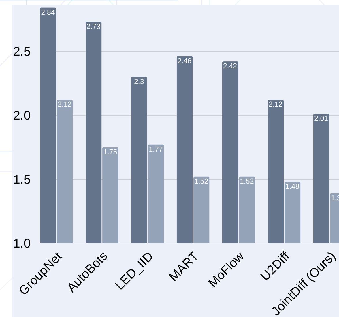
NBA (m) — SADE min / avg ↓
