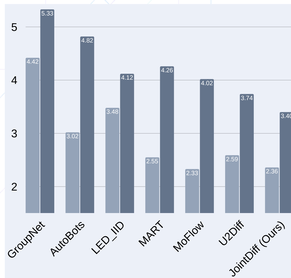
NFL (yards) — SADE min / avg ↓
