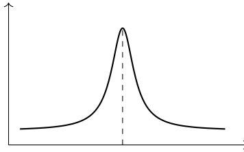
Figure 9: Schematic resonance peak in the invariant-mass distribution.
