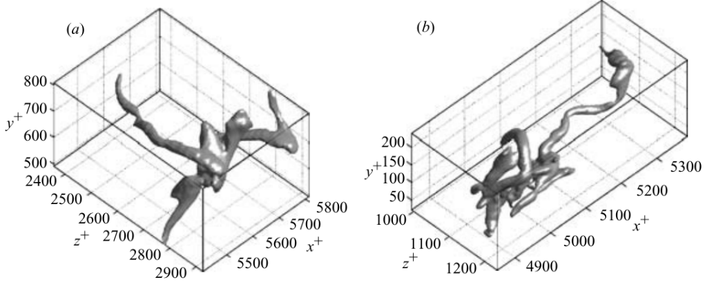
Figure 1: Representative detached (left) and tall attached (right) vortex clusters. The tall cluster is a multiscale connected object rather than one idealised vortex arch. Reproduced from figure 6 of del Álamo et al. [2006] .
