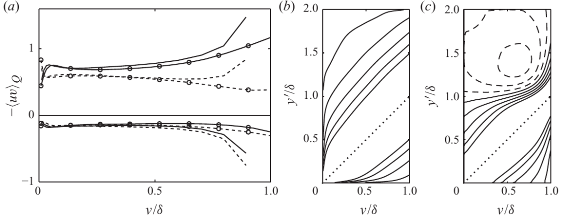
Figure 8: Quadrant contributions in a channel and a boundary layer (a), and wall-normal (b) and streamwise (c) large-scale channel correlations. Contours crossing y/\delta = 1 demonstrate centreline coupling. Reproduced from figure 5 of Jiménez et al. [2010].
