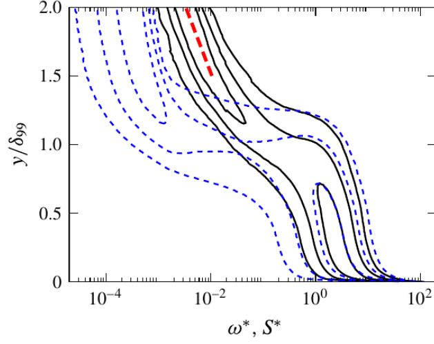
Figure 6: Joint wall-normal distributions of vorticity (blue dashed contours) and strain (black solid contours). Turbulent-level strain drops by more than one order of magnitude near the edge; the remaining weak potential branch follows the exponential decay marked in red. This is a separation of regimes, not continuous turbulent strain into the free stream. Reproduced from figure 20 of Borrell and Jiménez [2016] .
