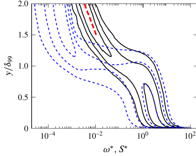
Figure 9: Joint wall-normal distributions of vorticity (blue dashed contours) and strain (black solid contours). Vorticity terminates rapidly, while strain extends into the free stream along the potential-flow decay marked in red. Reproduced from figure 20 of Borrell and Jiménez [2016] .
