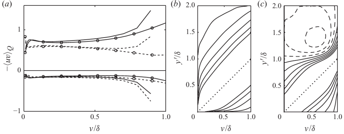
Figure 11: Quadrant contributions in a channel and a boundary layer (a), and wall-normal (b) and streamwise (c) large-scale channel correlations. Contours crossing y/\delta = 1 demonstrate centreline coupling. Reproduced from figure 5 of Jiménez et al. [2010].
