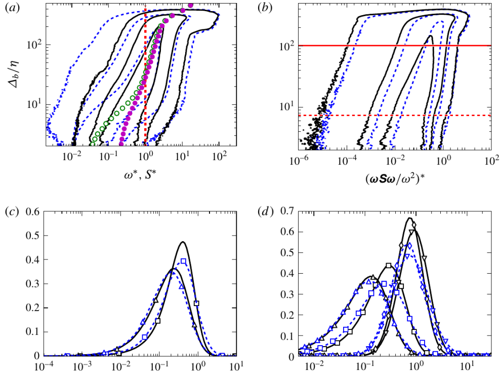
Figure 10: Conditional gradient statistics relative to the vorticity interface. Blue dashed curves in panels (c,d) are sampled at 7\eta and black solid curves at 100\eta . Their near collapse after local-strain normalisation shows that the interface retains the straining organisation of the core. Reproduced from figure 23 of Borrell and Jiménez [2016] .
