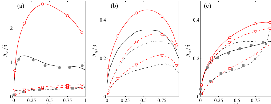
Figure 12: Integral correlation lengths for the three velocity components. In panel (a), the red channel curve for streamwise velocity continues to grow to y/\delta \simeq 0.5 , whereas the black boundary-layer curve levels off earlier. Reproduced from figure 10 of Sillero et al. [2014].
