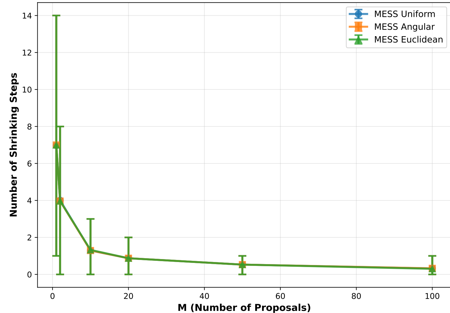
Mean Number of Shrinking Steps with 95% Credibility Intervals
