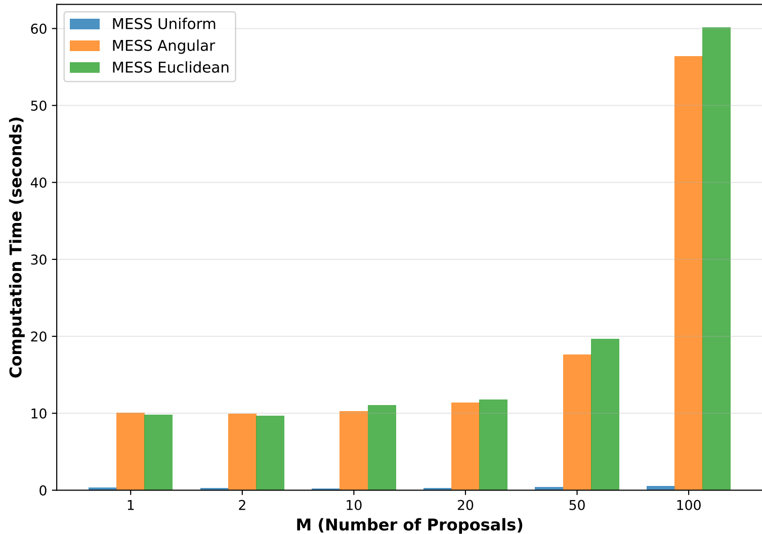
Computation Time Comparison
