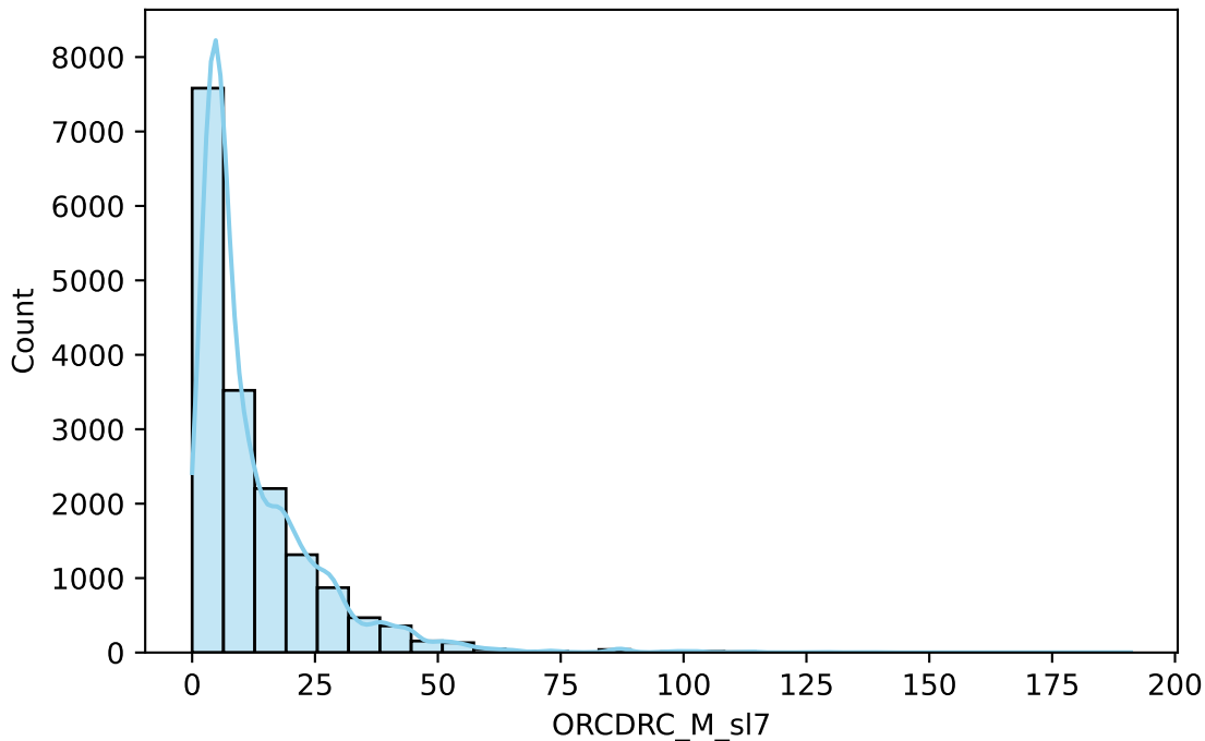
ORCDRC_M_sl7
