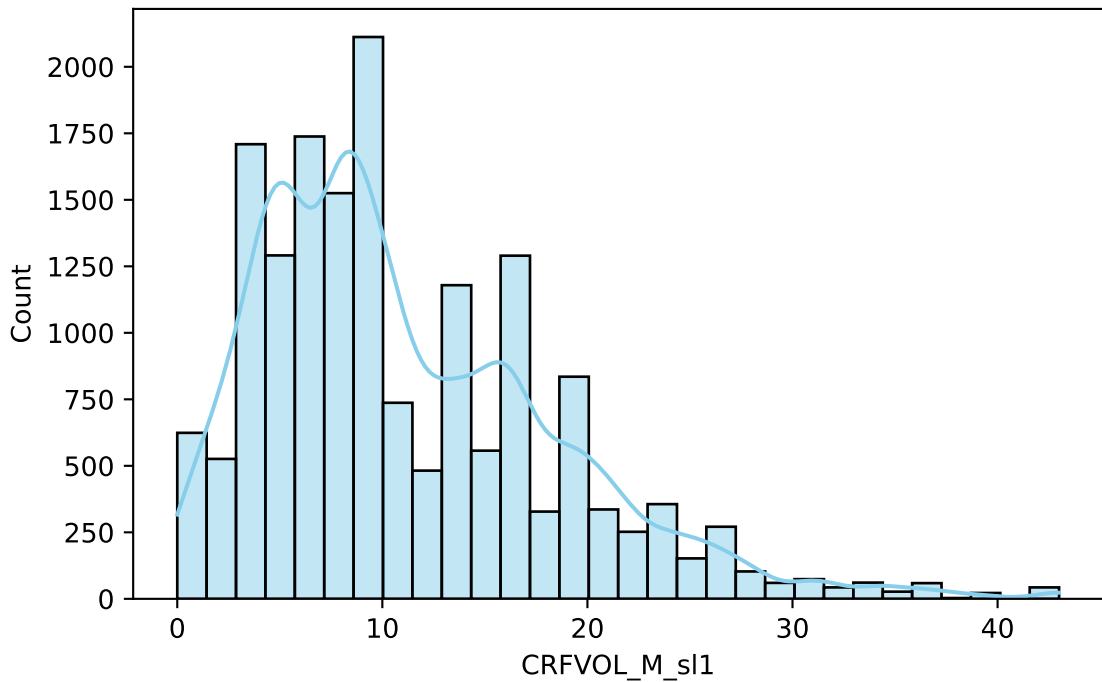
CRFVOL_M_sl1
