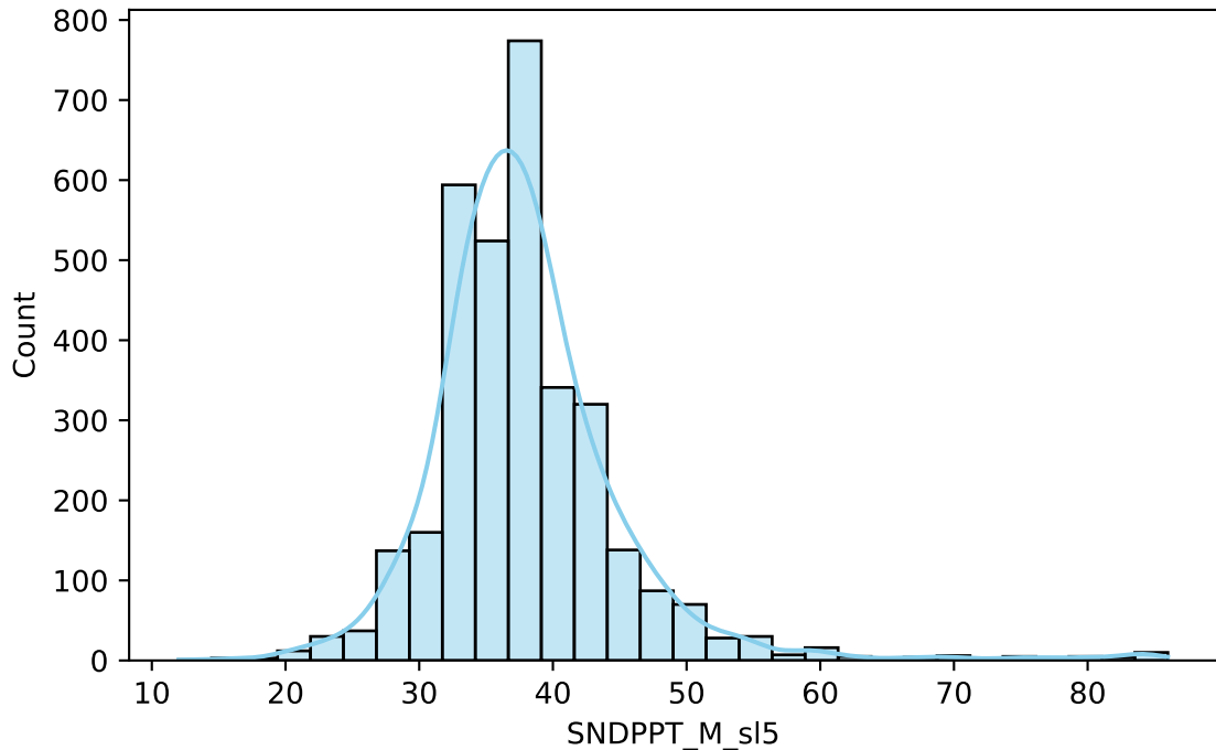
SNDPPT_M_sl5
