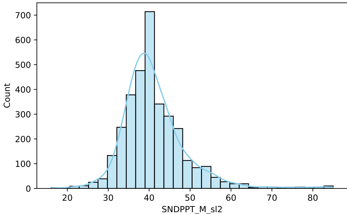
SNDPPT_M_sl2
