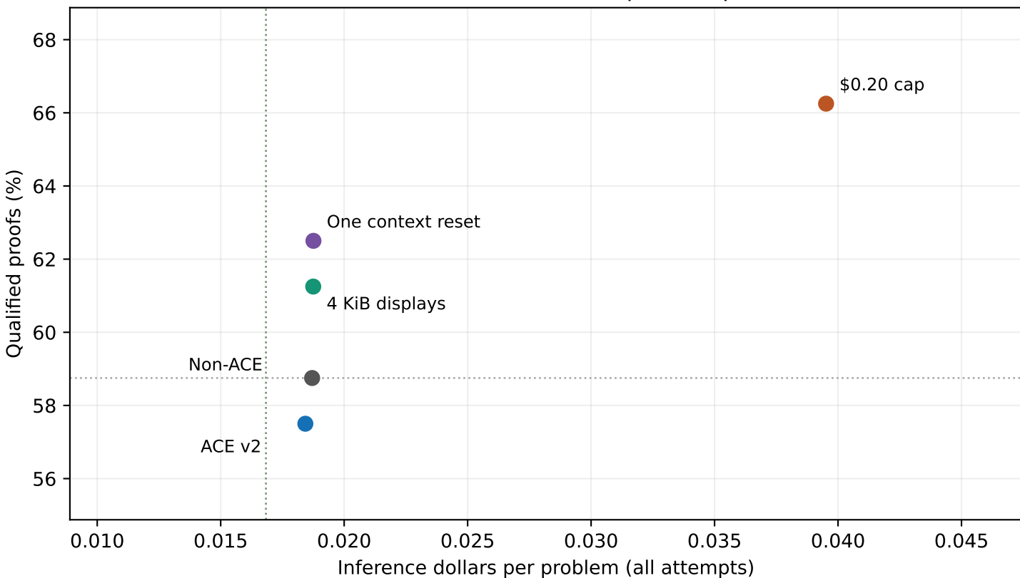
Observed cost and proof coverage; lower cost and higher coverage are preferable validationX: 40 theorems, 2 replicates per arm
