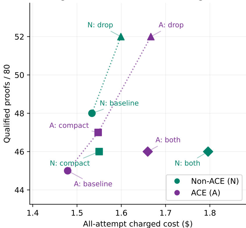
Each agent's observed cost / coverage frontier
