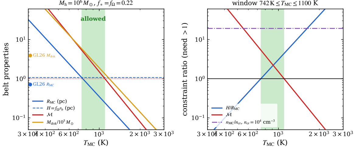
Figure 1. Left: cloud radius, Mach number and disk gas mass of the metal-poor belt as functions of the cloud temperature for M_h = 10^6 M_\odot , f_* = f_\Omega = 0.22 , x_{H_2} = \zeta = 1 . The dashed line is the disk half-thickness H = f_\Omega r_b , which does not depend on temperature; the dotted line marks \mathcal{M} = 1 . The corresponding GL26 values for the CO-cooled belt at 10 K are marked at the left edge for reference. Right: the two consistency ratios that must exceed unity, H/R_{MC} (clouds fit in the disk) and \mathcal{M} (clouds are supersonically turbulent), together with the ratio of the cloud density to a nominal LTE critical density of 10^4 \text{ cm}^{-3} . The shaded band is the allowed window of equation (29). The temperature of the H_2 -emitting gas is not a free parameter of the model but is confined to a factor of 1.5.
