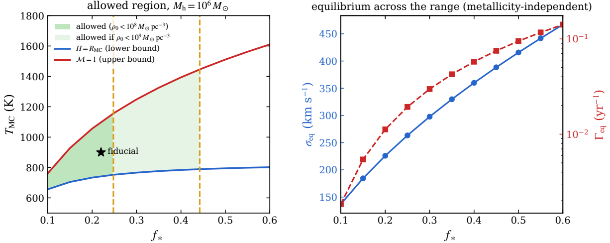
Figure 2. Left: the allowed region for the metal-poor engine in the plane of cusp flattening f_* (with f_\Omega = f_* , b = 1 ) and cloud temperature, for M_h = 10^6 M_\odot . The lower curve is the geometric requirement H = R_{MC} , the upper curve the sonic requirement \mathcal{M} = 1 . The vertical dashed lines mark the flattening at which the cusp central density reaches 10^8 and 10^9 M_\odot \text{pc}^{-3} ; the darker shading is allowed under the GL26 ceiling and the lighter shading under the relaxed ceiling appropriate to LRD cores. The AGN-dominance bound of GL26 does not appear because TDE momentum exceeds AGN radiation pressure everywhere on the plotted range at low metallicity. The star marks the fiducial solution. Right: the equilibrium dispersion and disruption rate across the same range of f_* ; both are set by the cusp alone and are independent of metallicity.
