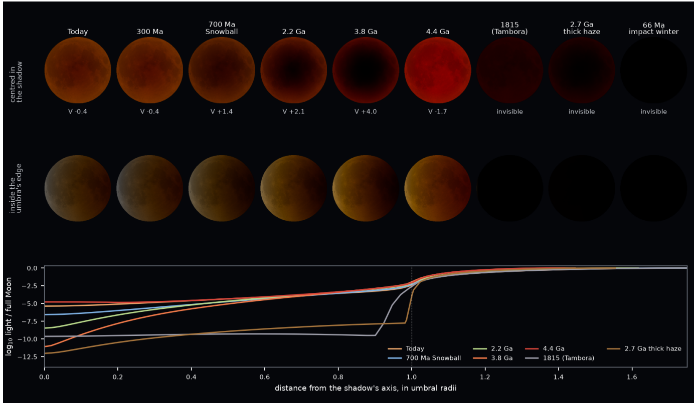
Figure 21: The Moon in the Earth's shadow at nine epochs, on today's lunar surface. Top: centered in the shadow, with its V magnitude, each drawn as the page draws it, for an eye adapted to that Moon's brightest part. Middle: just inside the umbra, its limb at 0.95 of the umbral radius, all at one exposure so their light compares: today's ozone leaves a cool gray-blue edge, the ozone-free Archean and Hadean edges are orange, and under the Tambora veil, the thick haze and the K–Pg soot the umbra is dark to its edge. Bottom: the light across the shadow, against the full Moon, with distance in units of each epoch's umbral radius.
