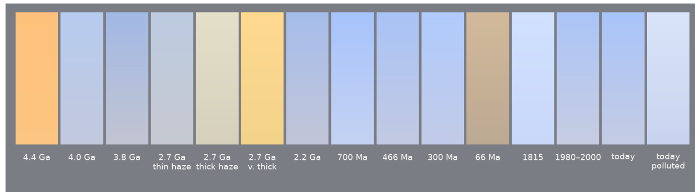
Figure 1. Mid-latitude noon sky at fifteen epochs, zenith (top) to horizon (bottom), oldest at left. Brightness shown relative to today's clean sky.
