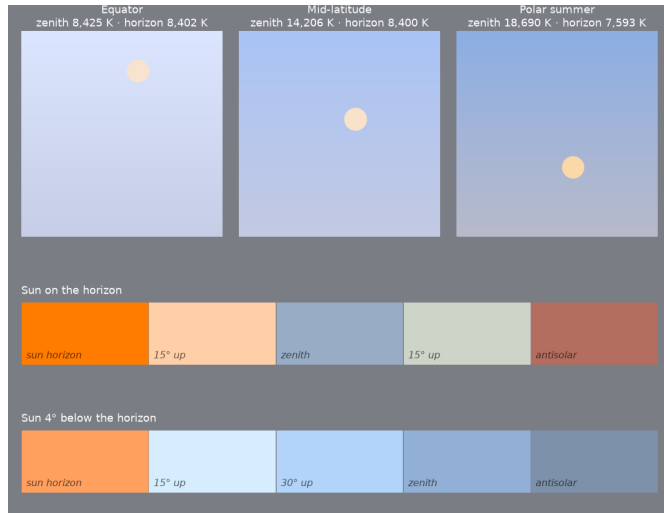
Figure 11: Ordovician meteor storm, ~466 Ma. Top: noon sky dome at the equator, mid-latitude and polar summer, zenith at top, horizon at bottom, Sun's disk in its own color. Below: sky from the solar horizon to the antisolar horizon with the Sun on the horizon and 4° below it.
