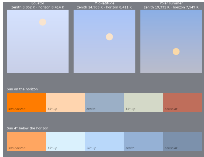
Figure 15: Geminga supernova, \sim 342 ka. Top: noon sky dome at the equator, mid-latitude and polar summer, zenith at top, horizon at bottom, Sun's disk in its own color. Below: sky from the solar horizon to the antisolar horizon with the Sun on the horizon and 4^\circ below it.
