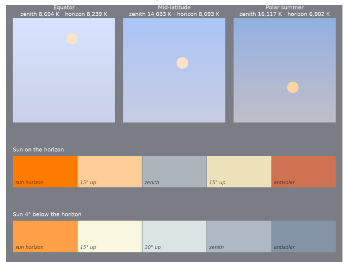
Figure 17: Ozone-hole spring. Top: noon sky dome at the equator, mid-latitude and polar summer, zenith at top, horizon at bottom, Sun's disk in its own color. Below: sky from the solar horizon to the antisolar horizon with the Sun on the horizon and 4^\circ below it.
