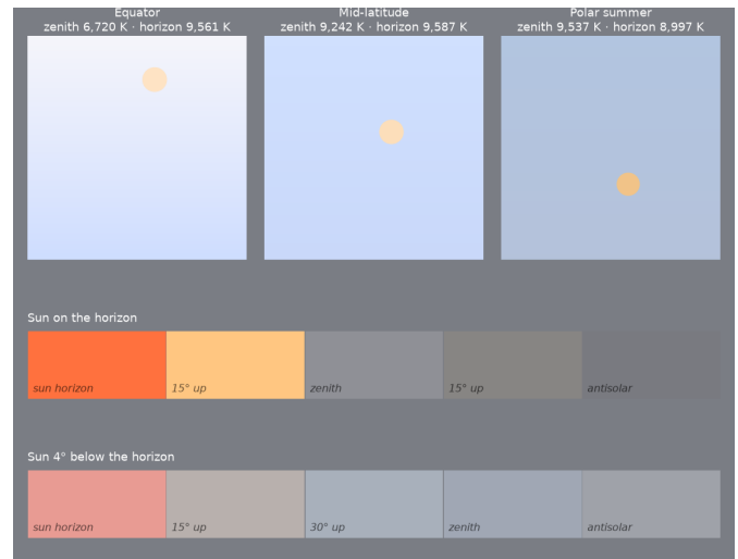
Figure 16: Volcanic year (Tambora 1815 / Toba-lite). Top: noon sky dome at the equator, mid-latitude and polar summer, zenith at top, horizon at bottom, Sun's disk in its own color. Below: sky from the solar horizon to the antisolar horizon with the Sun on the horizon and 4^\circ below it.
