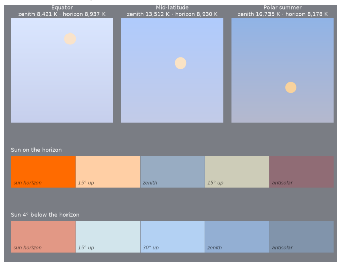
Figure 12: Carboniferous, ~300 Ma. Top: noon sky dome at the equator, mid-latitude and polar summer, zenith at top, horizon at bottom, Sun's disk in its own color. Below: sky from the solar horizon to the antisolar horizon with the Sun on the horizon and 4° below it.
