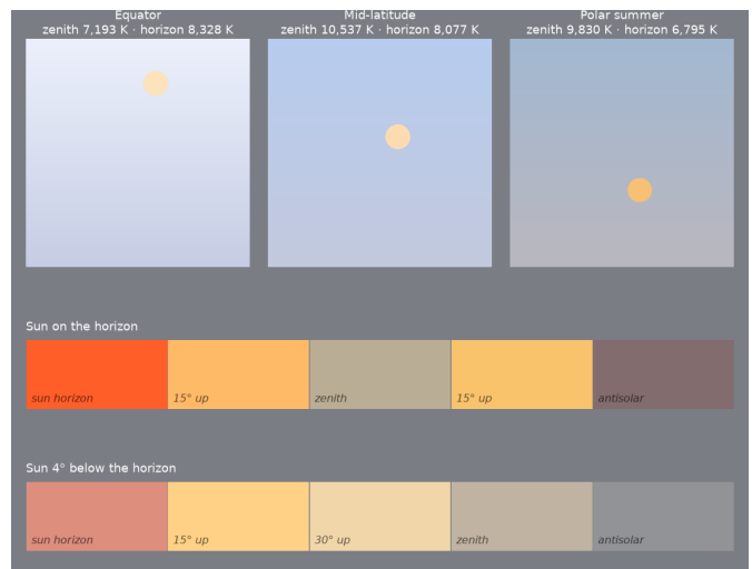
Figure 4: Late Hadean, ~4.0 Ga. Top: noon sky dome at the equator, mid-latitude and polar summer, zenith at top, horizon at bottom, Sun's disk in its own color. Below: sky from the solar horizon to the antisolar horizon with the Sun on the horizon and 4° below it.
