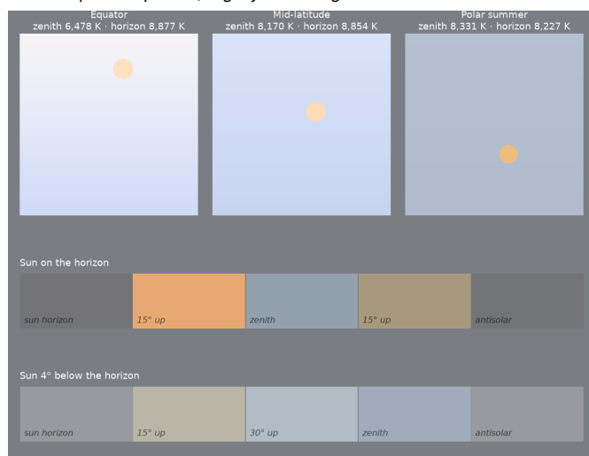
Figure 19: Modern, polluted megacity. Top: noon sky dome at the equator, mid-latitude and polar summer, zenith at top, horizon at bottom, Sun's disk in its own color. Below: sky from the solar horizon to the antisolar horizon with the Sun on the horizon and 4° below it.
