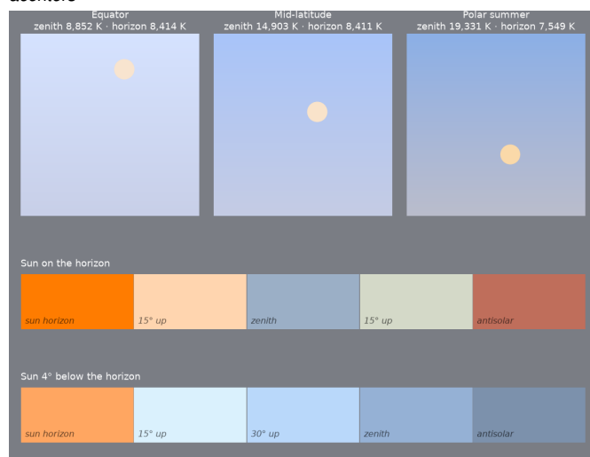
Figure 20: Year 2100. Top: noon sky dome at the equator, mid-latitude and polar summer, zenith at top, horizon at bottom, Sun's disk in its own color. Below: sky from the solar horizon to the antisolar horizon with the Sun on the horizon and 4° below it.
