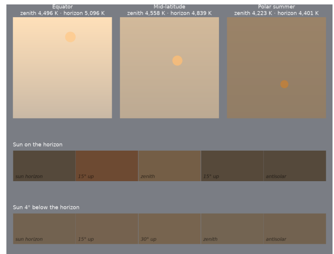
Figure 13: K-Pg impact winter, 66 Ma. Top: noon sky dome at the equator, mid-latitude and polar summer, zenith at top, horizon at bottom, Sun's disk in its own color. Below: sky from the solar horizon to the antisolar horizon with the Sun on the horizon and 4° below it.
