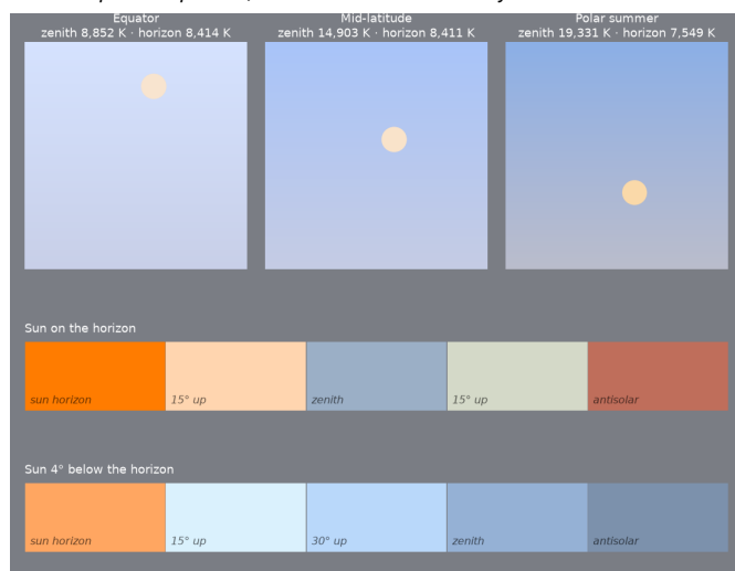
Figure 18: Modern, clean air. Top: noon sky dome at the equator, mid-latitude and polar summer, zenith at top, horizon at bottom, Sun's disk in its own color. Below: sky from the solar horizon to the antisolar horizon with the Sun on the horizon and 4° below it.
