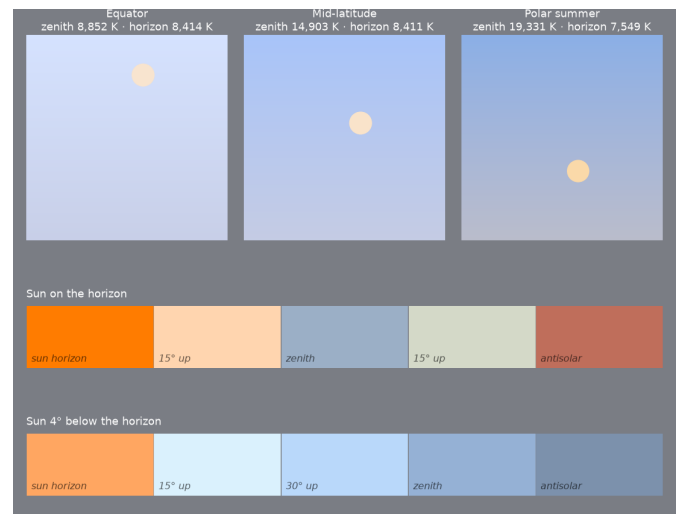
Figure 14: ζ Ophiuchi supernova, ~1.78 Ma. Top: noon sky dome at the equator, mid-latitude and polar summer, zenith at top, horizon at bottom, Sun's disk in its own color. Below: sky from the solar horizon to the antisolar horizon with the Sun on the horizon and 4° below it.
