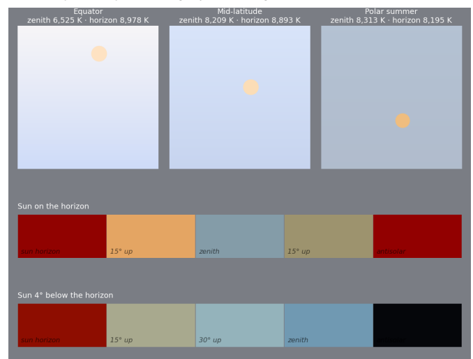
Figure 15: Modern, polluted megacity. Top: noon sky dome at the equator, mid-latitude and polar summer, zenith at top, horizon at bottom, Sun's disk in its own color. Below: sky from the solar horizon to the antisolar horizon with the Sun on the horizon and 4° below it.
