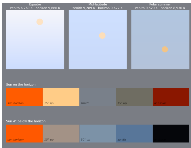
Figure 13: Volcanic year (Tambora 1815 / Toba-lite). Top: noon sky dome at the equator, mid-latitude and polar summer, zenith at top, horizon at bottom, Sun's disk in its own color. Below: sky from the solar horizon to the antisolar horizon with the Sun on the horizon and 4° below it.
