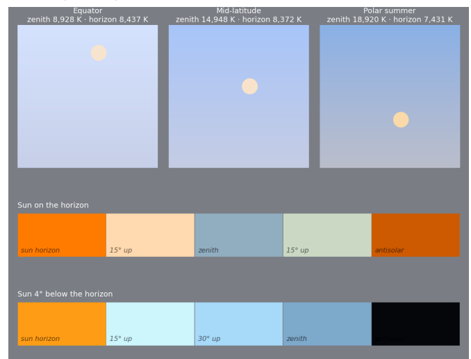
Figure 14: Modern, clean air. Top: noon sky dome at the equator, mid-latitude and polar summer, zenith at top, horizon at bottom, Sun's disk in its own color. Below: sky from the solar horizon to the antisolar horizon with the Sun on the horizon and 4° below it.
