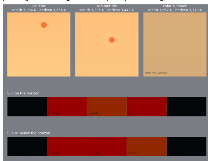
Figure 3: Early Hadean, \sim 4.4 Ga. Top: noon sky dome at the equator, mid-latitude and polar summer, zenith at top, horizon at bottom, Sun's disk in its own color. Below: sky from the solar horizon to the antisolar horizon with the Sun on the horizon and 4^\circ below it.
